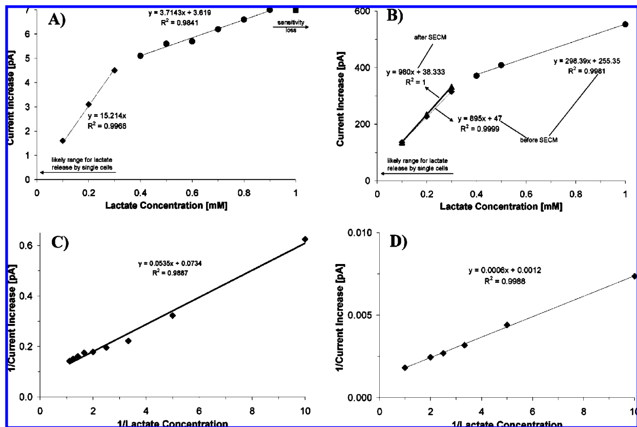
Figure 4. Amperometric calibrations of (A) electropolymerized and (B) cast LOx 25 \mu\text{m} UME biosensors, E = +0.6 V vs Ag/AgCl, 3 M KCl; additions up to 1 mM lactate in 50 mM phosphate buffer, pH 7. The sensors were calibrated for concentrations of up to 1 mM lactate and display two distinct linear regions: below 0.3 mM and above 0.4 mM, with the expected cellular lactate release range below 0.3 mM. The sensors retain lactate sensitivity upon being used in SECM experiments. Double-reciprocal plot representations of these amperometric calibrations: (C) the electropolymerized LOx sensor for which the corresponding data is shown in (A); (D) cast LOx sensor for which the corresponding data is shown in (B)—before use in SECM.
