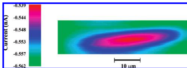
Figure 6. Glucose uptake profile for a single fibroblast. E = +0.6\text{ V} vs Ag/AgCl, 3 M KCl; 5 mM glucose in HBSS, pH 7.4; scanning speed 15 \mu\text{m/s} ; tip, GOx cast film on 25 \mu\text{m} UME biosensor; d = 10\text{ }\mu\text{m} from Petri dish; data have been corrected for background tilt in Origin Pro 7.5. The GOx cast 25 \mu\text{m} UME tip was positioned at 10 \mu\text{m} from the Petri dish by using approach curves (ACs).
