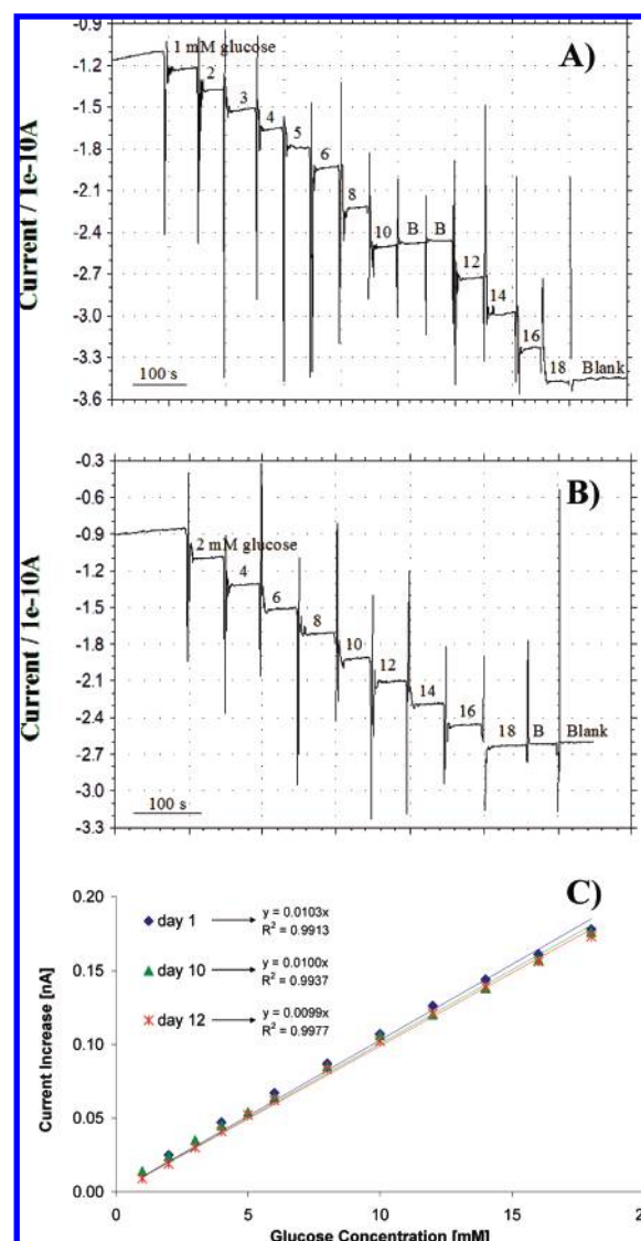
Figure 3. Amperometric calibrations of electropolymerized GOx 25 \mu m UME biosensors, E = +0.6 V vs Ag/AgCl, 3 M KCl; additions up to 18 mM glucose in 50 mM phosphate buffer, pH 7: (A) GOx UME sensors exhibit sensitivity to glucose prior to SECM experiments; (B) the sensors preserve the sensitivity to their analyte after being employed in extensive SECM experiments; (C) the electropolymerized GOx biosensors are stable in time when stored in 50 mM phosphate buffer, pH 7 at 4 °C for periods of at least 2 weeks; the same sensor shows almost identical sensitivity after 1, 10, and 12 days from the electropolymerization date. The data presented in this figure are for three distinct electropolymerized GOx sensors (one sensor for the data in (A), one sensor for the data in (B), and another sensor for the data in (C)).
