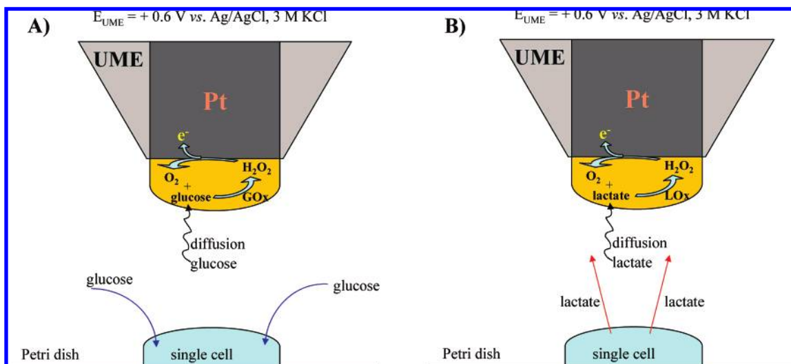
Figure 2. Enzyme-based UME biosensor. An enzyme layer (GOx (A) or LOx (B)) is deposited onto a 25 \mu\text{m} Pt UME by either electropolymerization or casting. The tip is rastered across the cell adhered to a Petri dish: (A) in the case of GOx it senses extracellular glucose depletion due to cellular uptake; (B) in the case of LOx it senses lactate production by the cell. The enzyme film breaks down the analyte, and the resulting \text{H}_2\text{O}_2 is oxidized at the underlying Pt UME. The arrows exiting the single cell denote lactate production (B).
