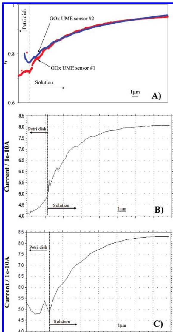
Figure 5. Approach curves (ACs) for 25 \mu\text{m} UME enzyme-based biosensors; E = +0.6\text{ V} vs Ag/AgCl, 3 M KCl; in 50 mM phosphate buffer, pH 7: (A) GOx electropolymerized sensors no. 1 (approach speed 1.5 \mu\text{m/s} ) and no. 2 (approach speed 3 \mu\text{m/s} ) yielded similar curves in 5 mM glucose, indicating reproducibility; (B) GOx cast sensor (5 mM glucose, approach speed 3 \mu\text{m/s} ); (C) LOx cast (0.5 mM lactate, approach speed 15 \mu\text{m/s} ). In all plots the vertical dashed line represents the point where the UME tip touches the Petri dish, coming from the right side (solution side).
