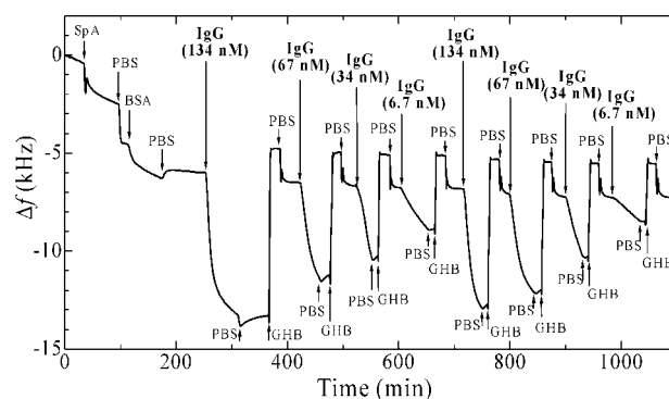
Figure 4. As-measured frequency response for an injection sequence. Arrows indicate the arrival time of solutions at the sensor cell.
