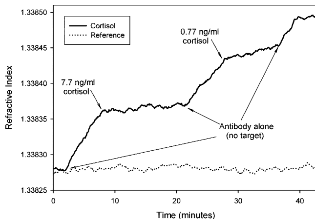
Figure 5. Detection of cortisol in laboratory buffer using the external, in-line filtering flow cell. Alternating flow through the external PEEK tube of buffer containing no cortisol (2, 22, and 36 min) with buffer containing 7.7 (28 nM) (8 min) or 0.77 ng/mL cortisol (2.8 nM) (28 min) demonstrated the detection of cortisol from the hollow fiber flow containing 1:15 000 diluted anticortisol antibody.
