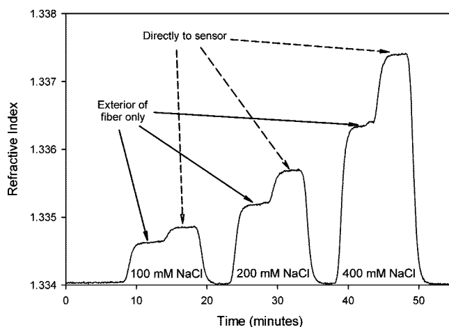
Figure 4. Small-molecule diffusion across the external, in-line filtering flow cell hollow fiber. PBS buffer solutions containing varying quantities (shown) of NaCl were flowed through the tubing external to the hollow fiber followed after 5 min with NaCl solution flowing directly over the sensor surface. The plateaus in signal RI represent the diffusion of NaCl at equilibrium for each condition. For external NaCl conditions, any NaCl that diffused into the hollow fiber resulted in an increase in RI on the SPR sensor. Flowing NaCl directly through the hollow fiber onto the sensor surface demonstrated the maximum RI change produced from each NaCl concentration.
