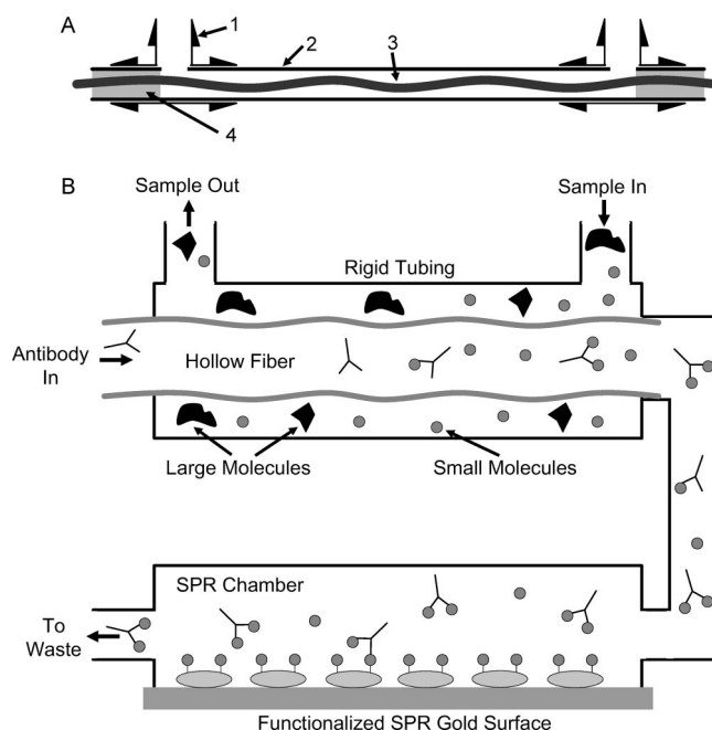
Figure 3. External, in-line filtering flow cell, which directs flow into the SPR system. (A) Construction of the in-line filtering flow cell required sliding a 1.6-mm Tee connector (1) (T210-1, Valve Plastics, Fort Collins, CO) over the ends of 0.75-mm inner diameter PEEK tube (2) (1533, Upchurch Scientific, Oak Harbor, WA), followed by drilling a hole into the PEEK tube to allow sample flow, and then sealing the PEEK tube to the tee with urethane adhesive (Lord Corp., Cary, NC). A hydrophilic hollow fiber (3) (Minntech, Minneapolis, MN) with a molecular weight cutoff of 20 000 was inserted into the PEEK tube, and both ends were sealed with urethane adhesive (4). Following sealing of the hollow fiber into the PEEK tube, the ends of the hollow fiber were cut flush with the tee preserving the opening to the hollow fiber. (B) Salivary samples were diluted 1:2 with buffer and flowed through tubing external to the hollow fiber. The antibody solution was flowed countercurrent through the hydrophilic hollow fiber and then through the SPR biosensor system. Diffusion may also be aided by bulk flow across the hollow fiber wall controlled by a pressure differential created by higher flow rates outside the hollow fiber (not drawn to scale).
