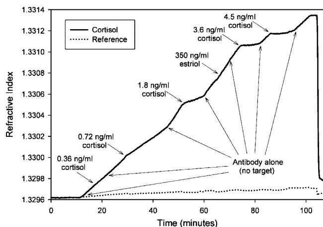
Figure 1. SPR competition assay for cortisol. The SPR biosensor surfaces were coated with either cortisol-conjugated BSA or BSA (reference channels). Mouse monoclonal anticortisol antibodies were introduced to the sensors at time = 12 min. Alternating pretreated samples with varying concentrations of cortisol were pulsed through the flow system. Reduction in binding slopes during antibody binding to the cortisol-conjugated BSA surface was used to measure cortisol. At time = 102 min, the sensors were washed with buffer alone, and then sensor surfaces were regenerated (at time = 104 min) using 100 mM glycine, pH 2.2. The data from three sensor channels were averaged for both the cortisol and reference measurements.
