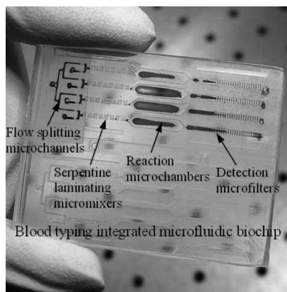
Figure 3. A biosensor chip for blood typing. 120 A single droplet of blood is split into four paths through a micromixer, reaction chamber and detection region. The blood type is read by eye. (Printed with permission from The Royal Society of Chemistry).
