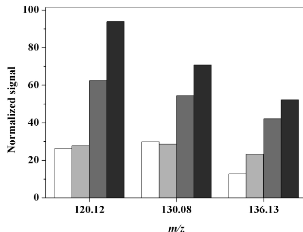
Figure 5. Characteristic TOF-SIMS fragments ( C_8H_{10}N^+ , C_9H_8N^+ , and C_8H_{10}NO^+ ) detected from the immobilized αCEA: white, bare SPGE; light gray, CNP-PEI/SPGE; dark gray, 50 μg/mL αCEA-immobilized CNP-PEI/SPGE; black, 1 mg/mL αCEA-immobilized CNP-PEI/SPGE.
