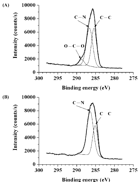
Figure 4. X-ray photoelectron spectra of the surfaces of the (A) antibody-deposited CNP-PEI/SPGE (50 μg/mL αCEA used) and the (B) CNP-PEI/SPGE.
