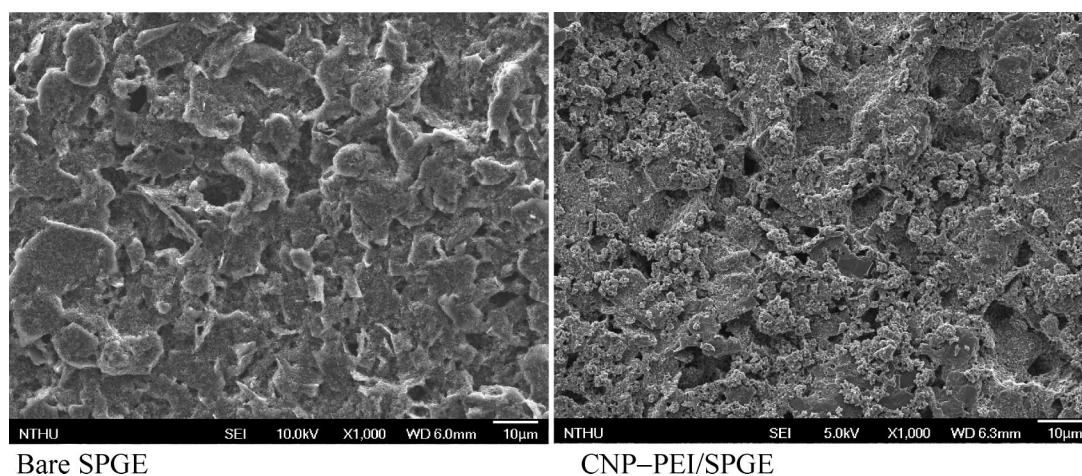
Figure 2. SEM images of the bare SPGE and the CNP–PEI-modified SPGE.
