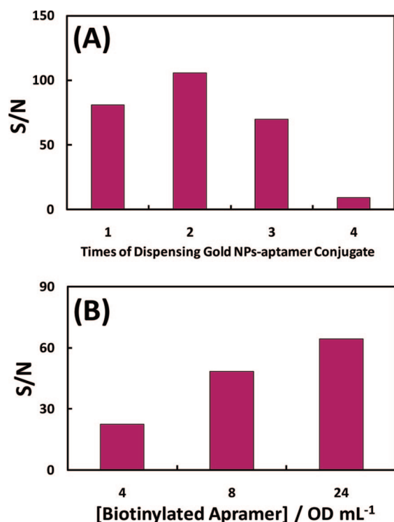
Figure 3. (A) Effect of dispensing times of gold NP-aptamer conjugate on the signal-to-noise ratio of the biosensor for 50 nM thrombin. Assay time, 10 min; sample solution was prepared with 15 \times \text{SSC} + 1\% \text{BSA} . (B) The effect of biotinylated aptamer concentration (immobilized on the test zone) on the signal-to-noise ratio of the biosensor for 50 nM thrombin. Assay time, 10 min; sample solution was prepared with 15 \times \text{SSC} + 1\% \text{BSA} ; times of dispensing gold NP-aptamer conjugate, 2.
