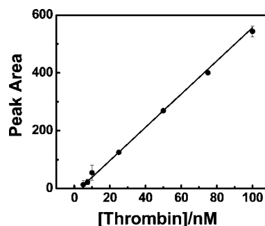
Figure 5. Calibration curve of the biosensor with different concentrations of thrombin in 15 \times \text{SSC} (1% BSA) buffer. Assay time, 10 min, sample volume, 120 \mu\text{L} .
