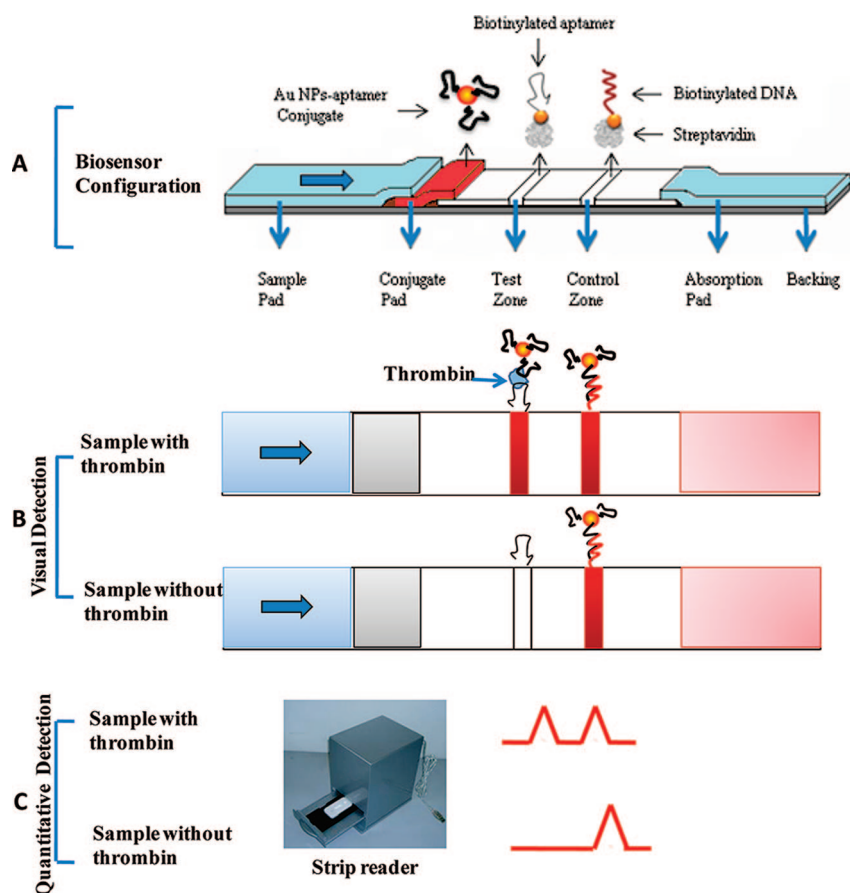
Figure 1. Schematic illustration of the configuration and measurement principle of the aptamer-based strip biosensor: (A) configuration of the biosensor; (B) the principle of visual detection in the presence and absence of thrombin; (C) quantitative detection with a portable strip reader.
