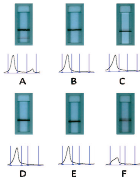
Figure 2. Typical photo images and recorded responses of the aptamer-based strip biosensor in the presence of (A) 50 nM thrombin, (B) 0 nM thrombin, (C) 500 nM HSA, (D) 500 nM IgG, (E) 500 nM IgM, and (F) 500 nM casein. Assay time, 10 min; sample solution was prepared with 15 \times \text{SSC} + 1% BSA; dispensing times of gold NP aptamer conjugate solution, 2; concentration of biotinylated aptamer for the preparation of test zone, 24 OD/mL.
