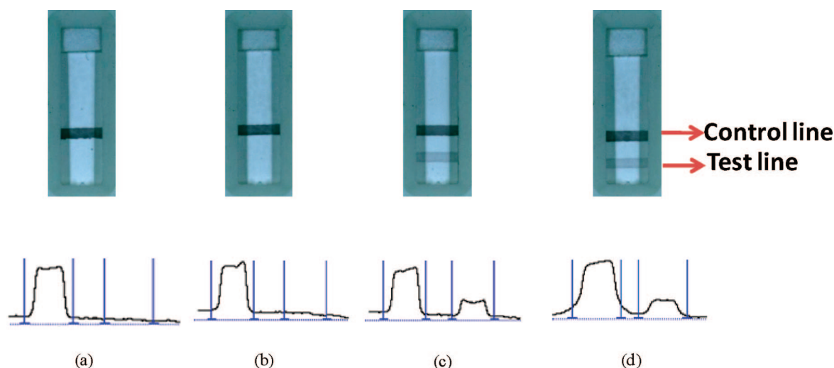
Figure 3. Typical photo images (top) and recorded response signals of DNAB with a portable strip reader after applying the sample solutions (bottom, left: optical response of the control line; right: optical response of the test line). (a): 0 nM target DNA; (b): 1000 nM noncomplementary DNA; (c): 100 nM target DNA; (d) 1000 nM noncomplementary target DNA+100 nM complementary target DNA. Assay time: 15 min; all sample solution were prepared with 4×SSC buffer.
