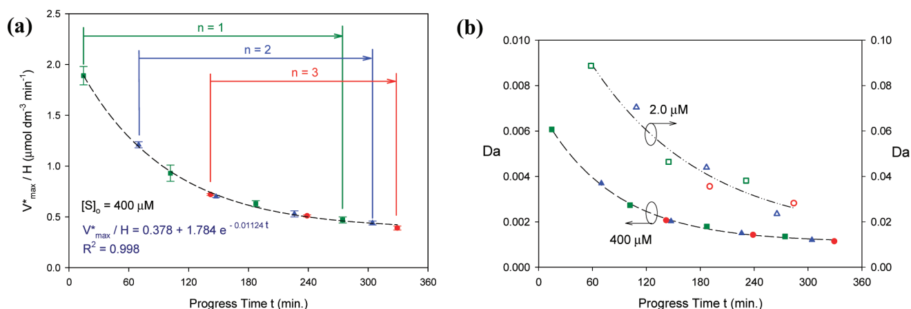
Figure 4. Stability of PST and its effect on the Damkohler number. (a) Deactivation curve of rat PST under saturating substrate condition. High substrate concentration ( 400 \mu\text{M} PAP) was used to give the characteristic curve of rat PST determined according to eq 9. Three data sets, dark-green rectangles, blue triangles, and red circles, were collected at different times (simultaneously and 1 and 2 h) after immobilization of PST. (b) Effect of substrate concentration and enzymatic activity on Da . Typical Da was obtained at space time \tau = 4 min. The curves decayed gradually due to the deactivation of enzyme. Dark-green squares, blue triangles, and red circles were recorded independently at different times after immobilization of PST. The upper (open symbols) and lower lines (solid symbols) represent low ( 2.0 \mu\text{M} ) and high ( 400 \mu\text{M} ) substrate concentration conditions, respectively.
