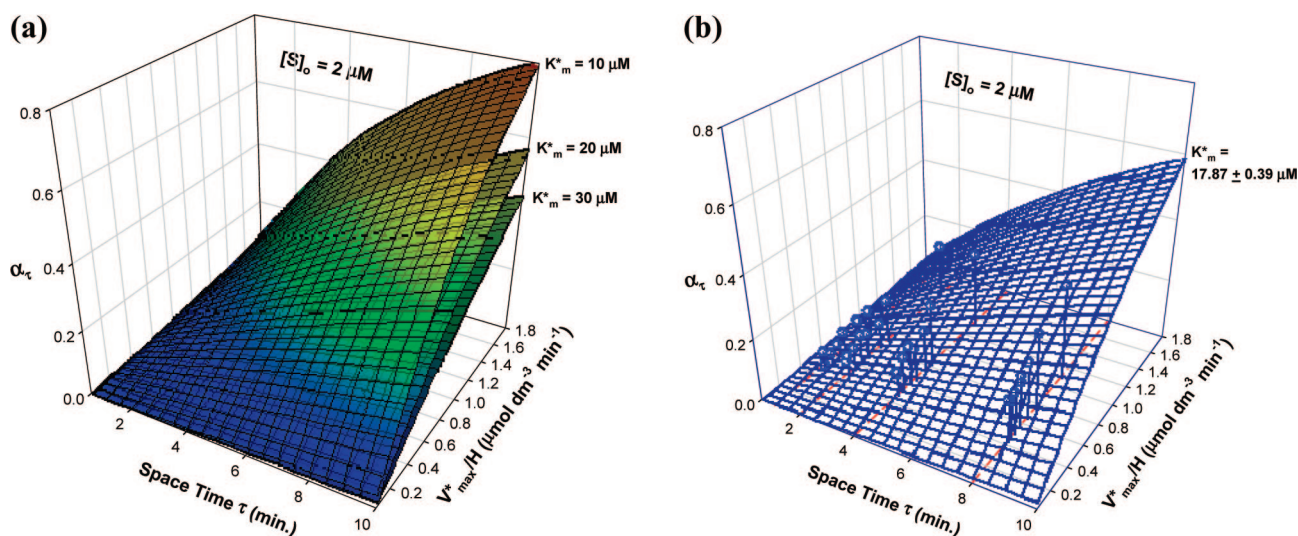
Figure 5. Curved surfaces of K_m^* in the space of \tau - V_{\max}^*/H - \alpha_\tau . (a) Computer-generated plots of eq 8 at moderate low concentration of substrate. Each K_m^* curved surface clearly separates one another at comparable low substrate concentration. (b) K_m^* curved surface produced by experimental data. The curved surface of K_m^* = 17.87 \pm 0.39 \mu\text{M} was generated through regression analysis of experimental data at [S]_0 = 2 \mu\text{M} .
