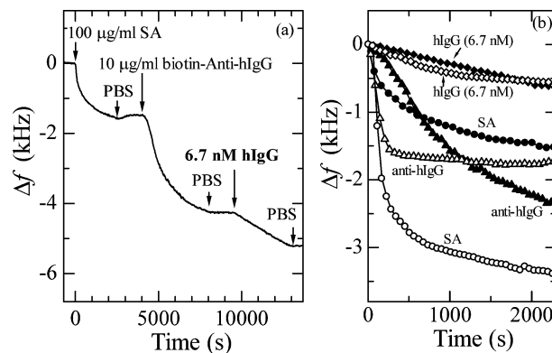
Figure 6. (a) A frequency response in a multi-injection measurement for a flow rate of 300 \mu\text{L}/\text{min} . (b) Comparison of binding curves for streptavidin on quartz (SA), anti-hIgG antibody on streptavidin (anti-hIgG), and hIgG on anti-hIgG antibody (hIgG) between two flow rates of 500 (open marks) and 300 (solid marks) \mu\text{L}/\text{min} .
