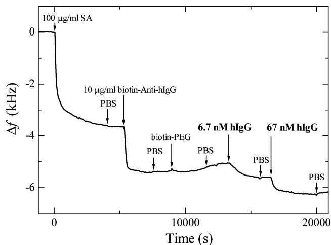
Figure 5. A frequency change observed in a multi-injection measurement. The flow rate is 500 \mu\text{L}/\text{min} .
