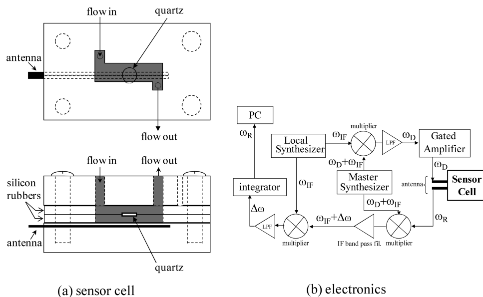
Figure 1. (a) Home-built sensor cell consisting of the line antenna, two Teflon covers, and two silicon rubbers (1 mm) sandwiching the 30 \mu\text{m} thick quartz plate. Upper and lower figures show the top and side views, respectively. Solutions flow in the shaded area. (b) The signal flow for measuring the resonance frequency of the quartz oscillator with the noncontacting manner.
