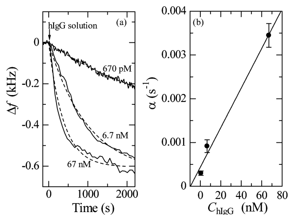
Figure 7. (a) Frequency changes with different concentrations of hIgG solutions observed at a flow rate of 500 \mu\text{L}/\text{min} . The broken lines are fitted theoretical functions (eq 4). (b) The relationship between the exponential coefficient \alpha versus the concentration of hIgG. The slope and intercept yield the kinetics constants.
