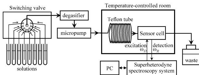
Figure 2. Home-built flow-injection-analysis system. The sensor cell is installed in the temperature control room where the temperature is kept at 37 °C.
