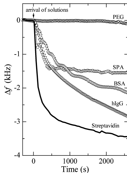
Figure 3. Frequency changes observed for injection of 100 \mu\text{g}/\text{mL} concentration proteins (PEG, SPA, BSA, hIgG, and streptavidin) in PBS.
