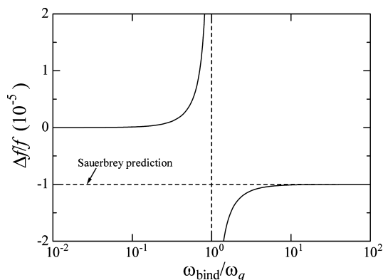
Figure 7. Dependence of the fractional change in the resonance frequency caused by the adsorption of proteins on the local resonance frequency \omega_{\text{bind}} at the binding pair (solid line). The horizontal broken line denotes the prediction by the Sauerbrey equation.
