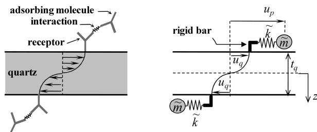
Figure 6. Continuum mechanics model for vibrations of a plate with point masses connected by the elastic springs.
