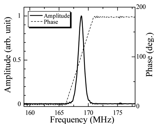
Figure 2. Resonance spectrum (solid line) and the phase change (broken line) of a 9.7 \mu\text{m} thick AT-cut quartz located in PBS measured by the line antennas contactlessly. Both quartz surfaces are exposed to the solution.
