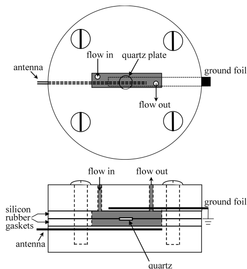
Figure 1. Top and side views of the home-built sensor cell. The two antenna wires are embedded in the bottom Teflon block, and the thin grounding foil is in the top Teflon block. The silicon rubbers sandwich the edge of a 9.7- \mu m thick quartz plate.
