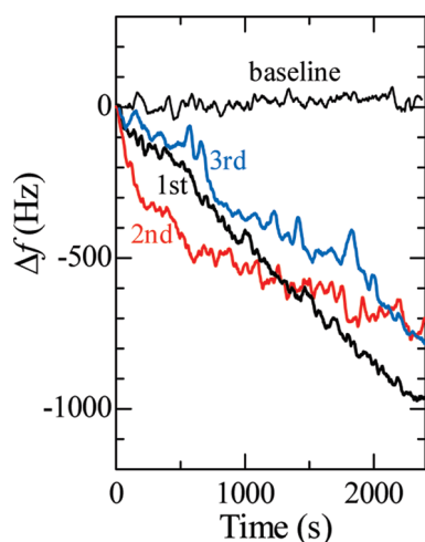
Figure 4. Resonance frequency changes caused by the injection of 0.5 pM hIgG solution. Three independent measurements are shown.
