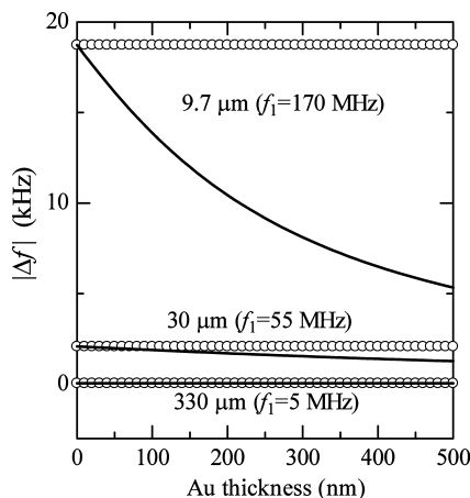
Figure 5. Influence of the gold electrode on the amount of the resonance frequency change caused by the adsorption of hIgG layers on both surfaces. The open circles denote the prediction by the Sauerbrey equation, and the solid lines are the analytical calculation for the five layer model.
