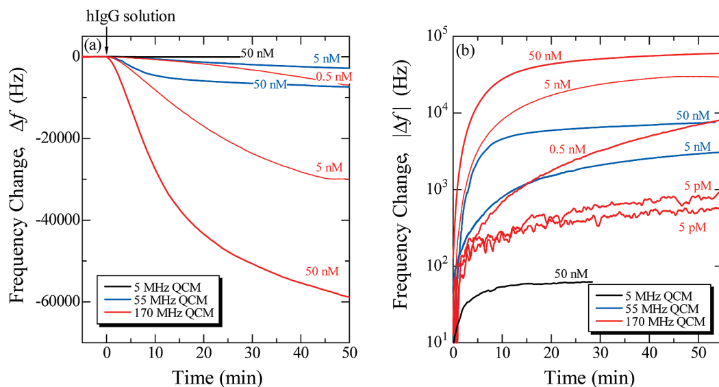
Figure 3. (a) Typical frequency changes caused by the injection of the hIgG solution detected by three electrodeless QCMs. (b) Logarithmic resonance-frequency change during the injection of the hIgG solution. For the 5 pM hIgG solution, two independent measurements are shown.
