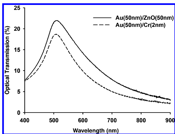
Figure 3. The measured transmission spectrum of the Au/Cr layer (dash line) and the Au/ZnO layer (solid line).
