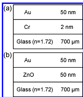
Figure 1. Schematic diagram of the thin film structure (not drawn to scale) in (A) Au/Cr and (B) Au/ZnO. The refractive indices of a ZnO film and a Cr film are 1.98 and 4.14, respectively.
