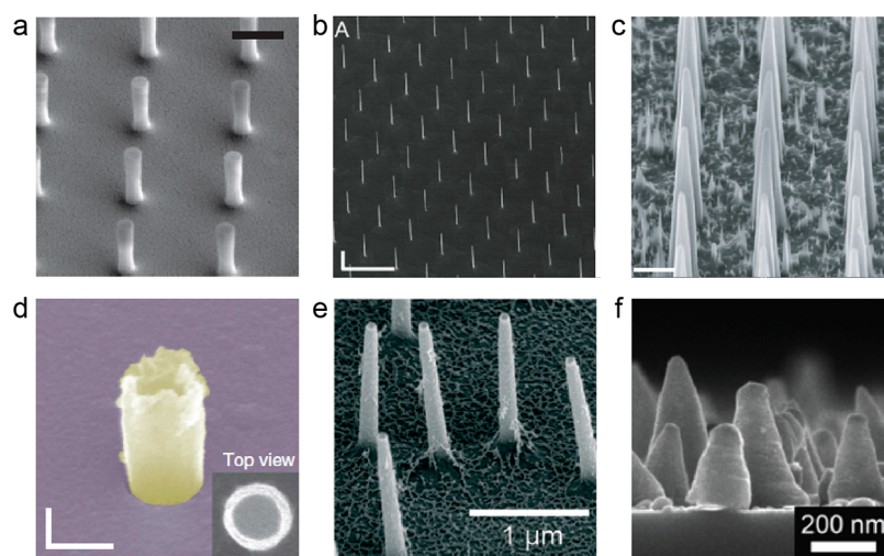
Figure 1. Overview of vertical nanostructures including (a) nanopillars, 23 (b) nanowires, 27 (c) nanoneedles, 11 (d) nanotubes, 55 (e) nanostraws, 40 and (f) nanocones. 57 The diameter, height, and aspect ratio of the vertical nanostructures are as follows: (a) 150 nm, 1.4 \mu\text{m} , 9; (b) 91 nm, 11 \mu\text{m} , 120; (c) 600 nm, 9 \mu\text{m} , 15; (d) 181 nm, 500 nm, 3; (e) 100 nm, 1.5 \mu\text{m} , 15; (f) 50 nm, 200 nm, 4. Scale bars are as follows: (a) 1 \mu\text{m} , (b) 500 nm, (c) 2 \mu\text{m} , (d) 200 nm. Reprinted with permission from the following: ref 23, Copyright 2015 Nature Publishing Group; ref 27, Copyright 2012 IOP Publishing Ltd.; ref 11, Copyright 2015 Nature Publishing Group; ref 55, Copyright 2014 Nature Publishing Group; ref 40, Copyright 2016 Royal Society of Chemistry; ref 57, Copyright 2014 Springer Nature.
