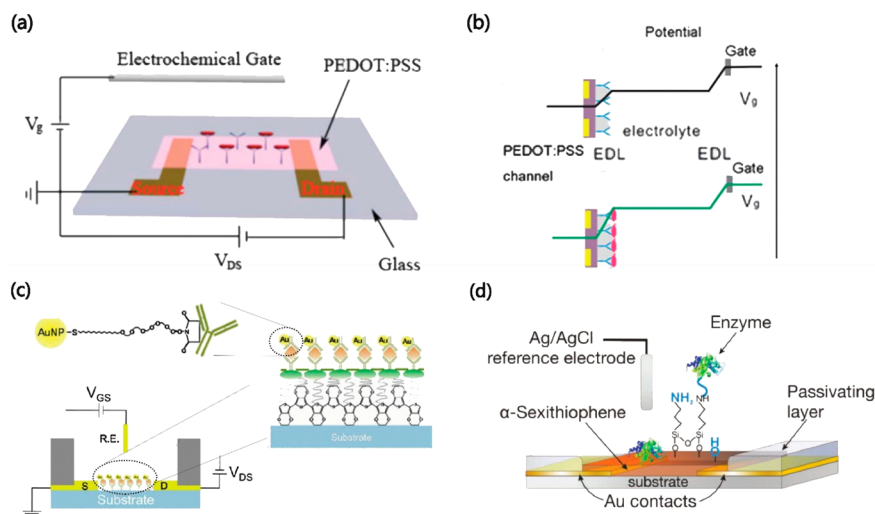
Figure 1. (a) Device structure of an OEFT sensor for capture of E. coli bacteria; (b) potential drop profile before and after the capture of bacteria on the PEDOT:PSS surface. Reproduced with permission from ref 8. Copyright 2012 Royal Society of Chemistry. (c) OEFT based immunosensor with the signal amplified by linked gold nanoparticles. Reproduced with permission from ref 10. Copyright 2010 Elsevier. (d) Structure of a biofunctional EGOFT with covalently bonded enzymes on the surface of \alpha -sexithiophene thin film. Reproduced with permission from ref 11. Copyright 2012 Wiley.
