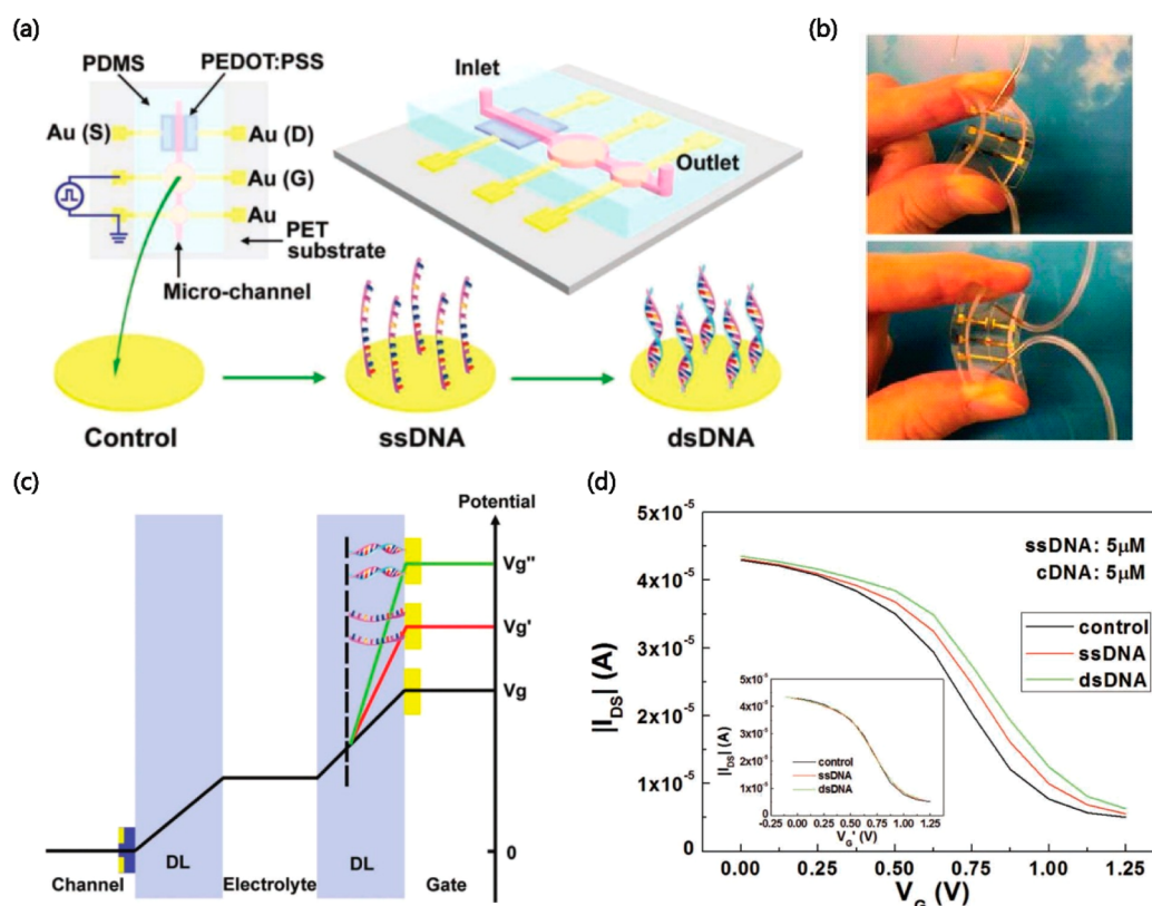
Figure 4. (a) Schematic of an OEFT integrated in a microfluidic system, with DNA molecules on gate electrodes. (b) Photograph of a flexible device bent to different directions. (c) Potential drop profiles with the immobilization of probe (red line, V_{g'} ) and target (green line, V_{g''} ) DNA molecules. (d) Transfer characteristics of the OEFT before and after the modification and hybridization of DNA on gold electrode. Reproduced with permission from ref 23. Copyright 2011 Wiley.
