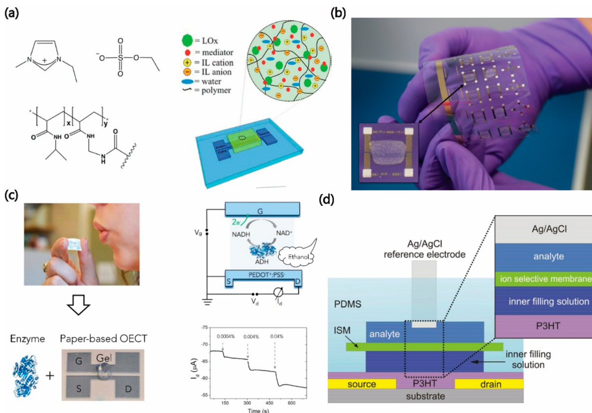
Figure 3. (a) The chemical structure and schematic description of components in ionic-gel electrolytes. Reproduced with permission from ref 19. Copyright 2012 Royal Society of Chemistry. (b) Photograph of the screen-printed all-solid-state OECT on flexible substrates. Reproduced with permission from ref 20. Copyright 2015 Materials Research Society. (c) Breathing on the enzyme-embedded OECT on paper, associated with the mechanism and the drain current response of the device toward exposure to ethanol. Reproduced with permission from ref 21. Copyright 2016 Springer Nature. (d) Schematic structure of the EGOFET integrated with an ion selective membrane. Reproduced with permission from ref 22. Copyright 2013 Wiley.
