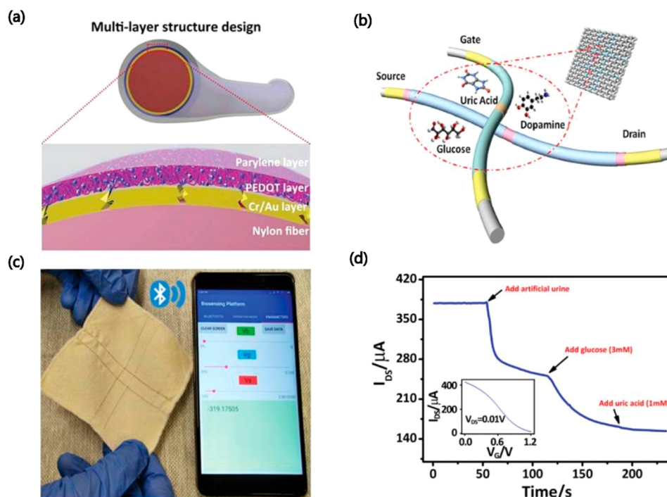
Figure 9. (a) The design of multilayer electrodes in OEFTs prepared on nylon fibers. (b) Illustration of OEFT integrated into textiles as fabric sensor for different sensing scenarios. (c) Photograph of fabric OEFTs controlled by a mobile phone through Bluetooth. (d) Channel current responses of a fabric OEFT integrated in a diaper to artificial urines with the addition of glucose and uric acid (interference). Reproduced with permission from ref 45. Copyright 2018 Wiley.
