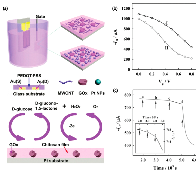
Figure 7. (a) OECT-based glucose sensor modified with multiwall carbon nanotubes (MWCNTs) or Pt nanoparticles. (b) Transfer characteristics of a Pt nanoparticle functionalized OECT in (I) blank and (II) 100 μM glucose PBS solutions. (c) Channel current responses to glucose additions with concentrations of a = 0.005, b = 0.05, c = 0.5 and d = 5 μM. Reproduced with permission from ref 36. Copyright 2011 Wiley.
