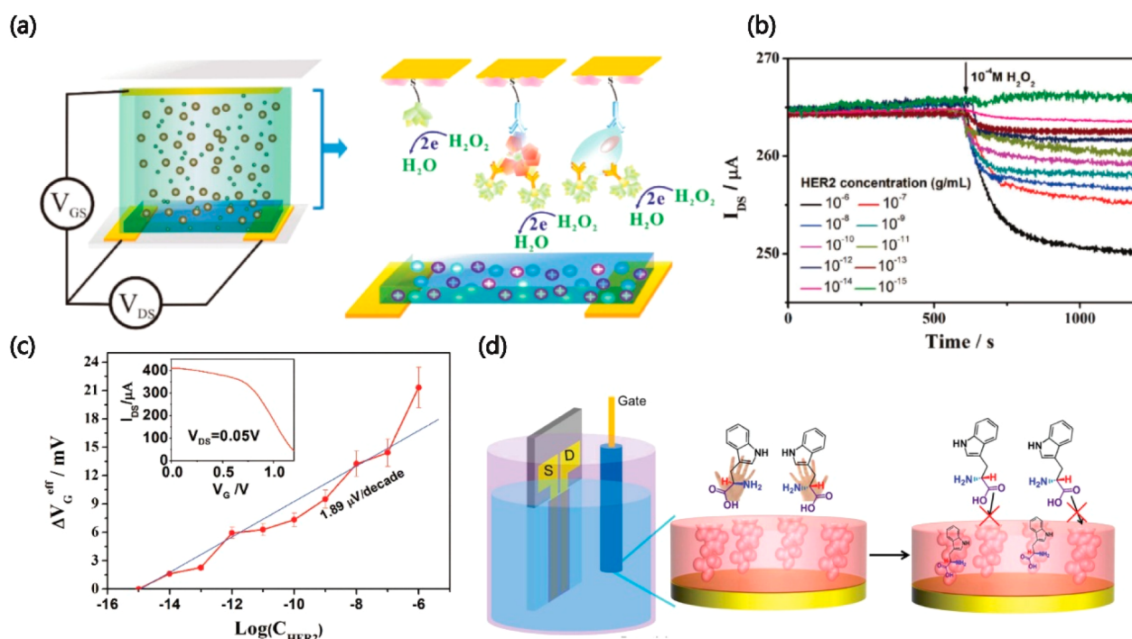
Figure 5. (a) Gate electrode modification of OECTs for protein or cell detection. (b) Channel current responses and (c) effective gate voltage changes of OECTs exposed to cancer cell biomarkers with different concentrations. Reproduced with permission from ref 26. Copyright 2017 Wiley. (d) Chirality detection of amino acid enantiomers by OECTs modified with molecularly imprinted polymer films. Reproduced with permission from ref 27. Copyright 2018 Elsevier.
