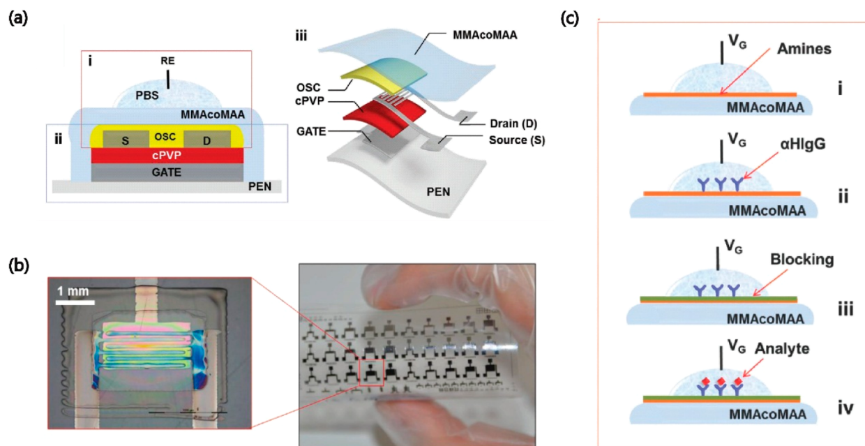
Figure 8. (a) Design of a flexible OTFT biosensor. (b) Photograph of printed OTFT arrays. (c) Functionalization processes at the insulator/electrolyte interface. Reproduced with permission from ref 41. Copyright 2014 Wiley.
