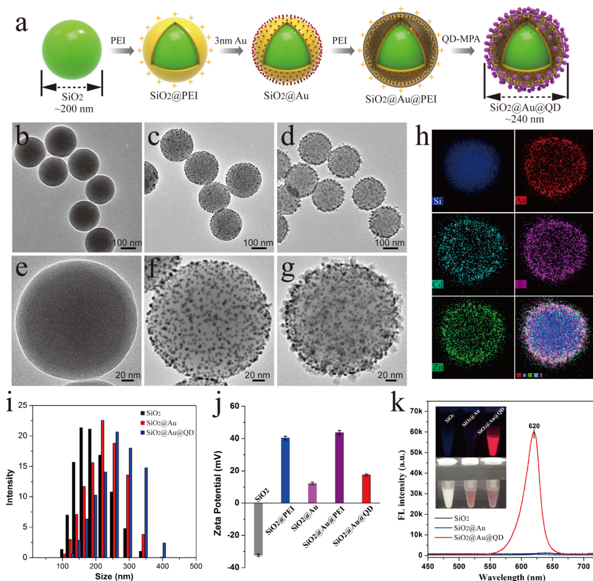
Figure 1. (a) Sequential process for fabricating dual-mode SiO 2 @Au@QD fluorescent labels. TEM images of (b) SiO 2 , (c) SiO 2 @Au, and (d) SiO 2 @Au@QD, with their corresponding magnified TEM images of a single particle in (e), (f), and (g), respectively. (h) Elemental mapping images of a single SiO 2 @Au@QD NP. (i) DLS distribution of SiO 2 (black), SiO 2 @Au (red), and SiO 2 @Au@QD (blue). (j) \zeta -Potentials of the products from each stage. (k) Fluorescence spectra of SiO 2 , SiO 2 @Au, and SiO 2 @Au@QD under UV light. (Inset) Photographs of these particles under UV light (above) and visible light (below).
