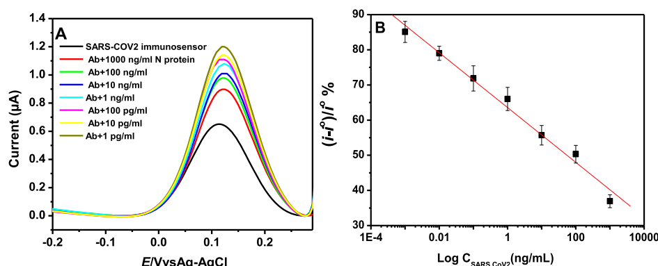
Figure 4. Square wave voltammograms of the SARS-CoV-2 (A) immunosensors before and after binding with different concentrations of nucleocapsid protein mixed with 10 \mu\text{g/mL} nucleocapsid antibody solution. The calibration plot of SARS-CoV-2 (B) detection [plot of the logarithm of the antigen concentration vs the percentage change in the SWV peak current before and after binding (i - i^0)/i^0 %]. The error bars show the standard deviations of three measurements.
