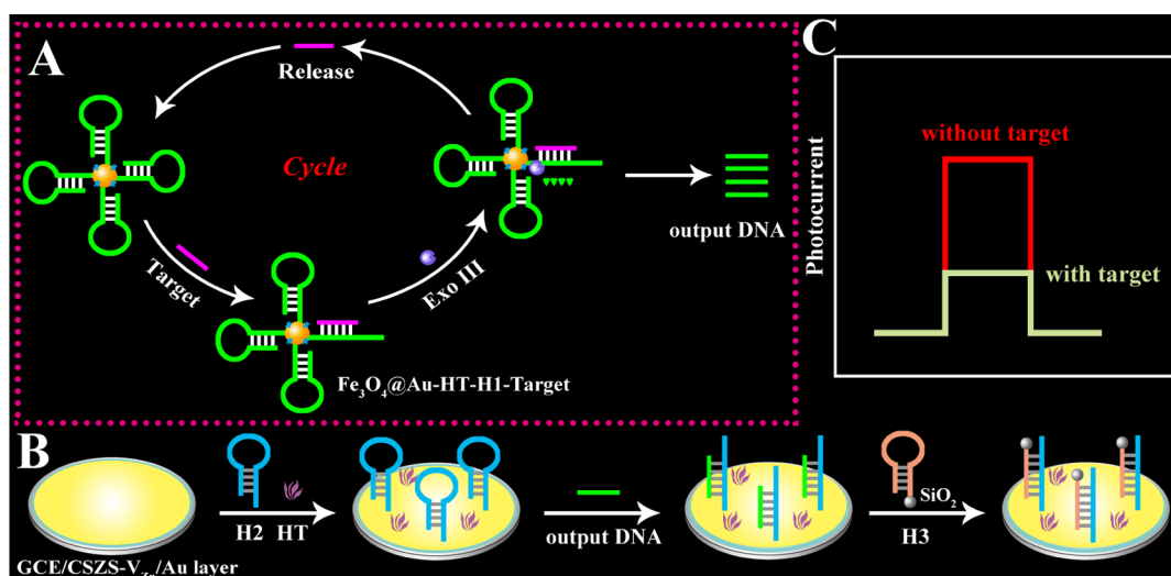
Scheme 1. Schematic Illustration of (A) Highly Efficient Exo III-Assisted Cycling Amplification, (B) Assembly of the PEC Biosensor, and (C) Photocurrent Response with or without Target miRNA-122
