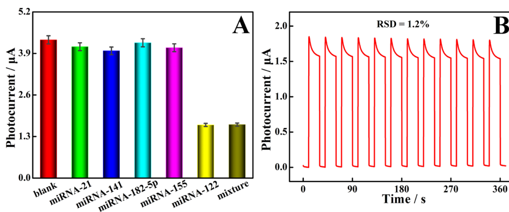
Figure 6. (A) Selectivity of the proposed biosensor to the blank control group and different substances: miRNA-21, miRNA-141, miRNA-182-5p, miRNA-155, the mixture, and target. (B) Stability of the PEC biosensor in the presence of 100 fM miRNA-122 under consecutive periodic “off–on–off” light for 12 cycles.
