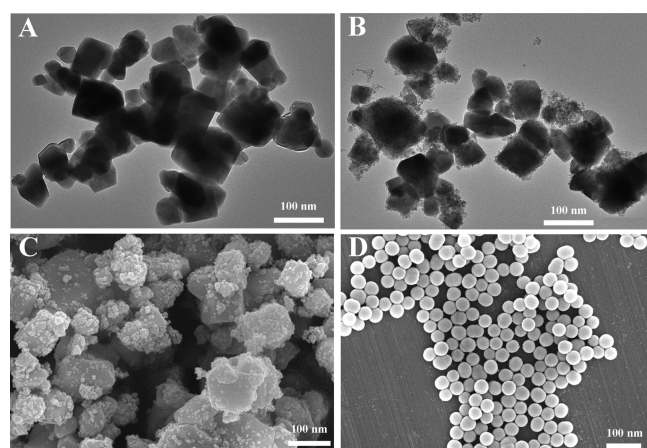
Figure 1. TEM images of ZnS- \text{V}_{\text{Zn}} (A) and CSZS- \text{V}_{\text{Zn}} (B) and SEM images of CSZS- \text{V}_{\text{Zn}} (C) and \text{SiO}_2 NPs (D).
