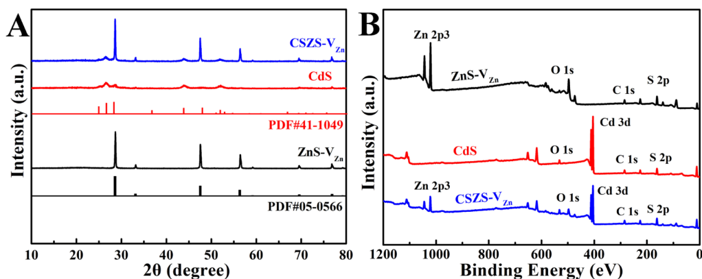
Figure 2. XRD patterns (A) and XPS survey spectra (B) of CdS, ZnS-V Zn , and CSZS-V Zn .
