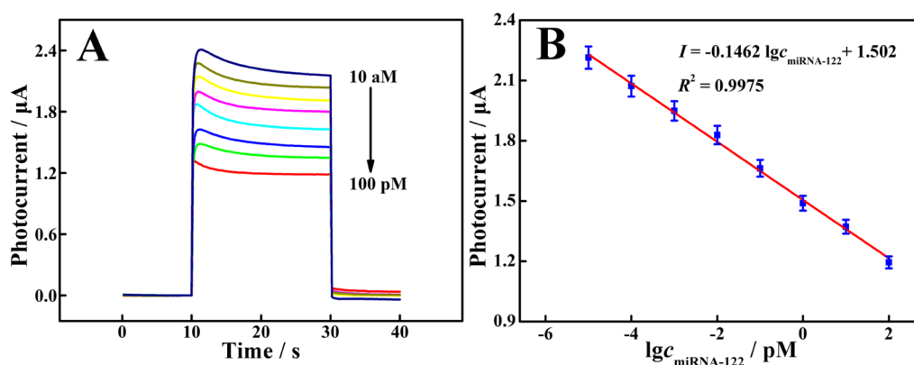
Figure 5. (A) Photocurrent response of the biosensor with different miRNA-122 concentrations: 10 aM, 100 aM, 1 fM, 10 fM, 100 fM, 1 pM, 10 pM, and 100 pM. (B) Corresponding linear calibration curve for miRNA-122 detection at various concentrations.
