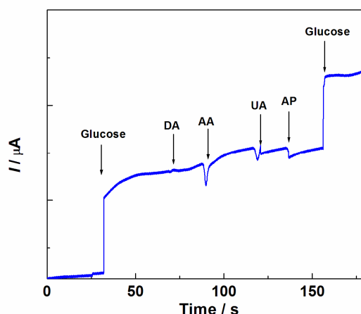
Figure 4. Amperogram response to 0.2 mM of glucose at -0.463 V in the presence of different interferents including 0.2 mM DA, 0.3 mM AA, 0.5 mM UA, and 0.5 mM AP.
