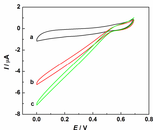
Figure 5. CVs of BOD-CNDs/GC electrode under nitrogen (curve a), air (curve b), oxygen (curve
