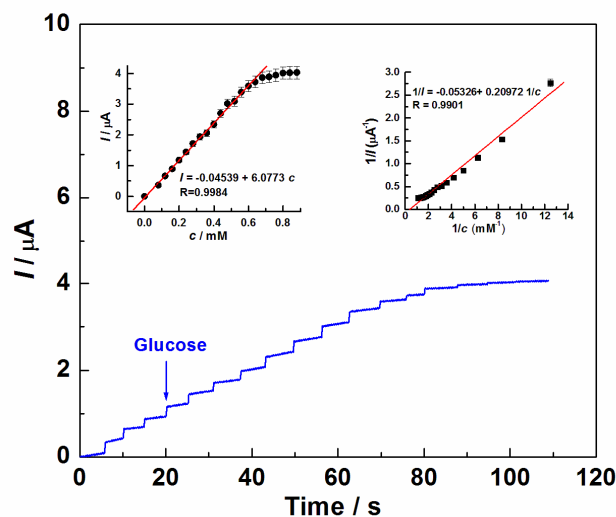
Figure 3. Chronoamperometric i - t response of GOx-CNDs/GC electrode to glucose with various concentrations in \text{N}_2 -saturated phosphate buffer at -0.463 \text{ V} . Inset: the corresponding calibration plot (current versus concentration, left panel) and the plot of 1/I_{\text{ss}} against 1/c (current -1 versus concentration -1 , right panel).
