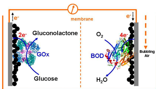
Scheme 1. Illustration of the fabricated DET-type glucose/air BFC.
