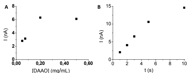
Figure 2: Effect of DAAO concentration on 1 mM D-Met amperometric signal. Conditions: 5 mM sodium phosphate buffer pH 8.0, detection potential + 0.70 V (A). Effect of injection time on 0.50 mM D-Met amperometric signal. Conditions: 5 mM sodium phosphate buffer pH 8.0, 0.50 \text{ mg} \cdot \text{mL}^{-1} DAAO, detection potential + 0.70 V (B). Electrokinetic conditions as in Figure 1.
