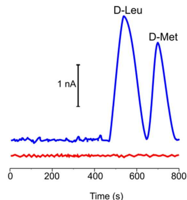
Figure 5: Microchip electropherograms corresponding to the reaction of: 0.50 \text{ mg} \cdot \text{mL}^{-1} DAAO with a mixture of 0.50 mM D-Leu and 0.30 mM D-Met (blue) and 0.50 \text{ mg} \cdot \text{mL}^{-1} DAAO with a mixture of 0.50 mM L-Leu and 0.30 mM L-Met (red). Conditions: borate buffer (20 mM pH 10.0), detection potential +0.70 V. Electrokinetic conditions as in Figure 1.
