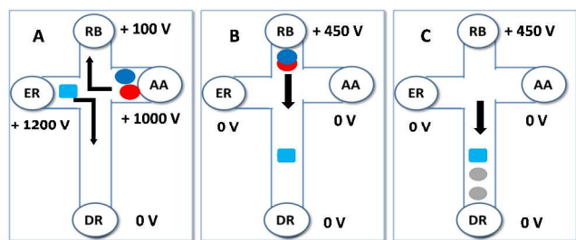
Figure 1: Electrochemical microfluidic strategy: enzyme and D-AAs electrokinetic injection for 5 s (A), enzyme and D-AAs electro-focusing (B) and D-AAs separation and in-channel enzymatic reaction and hydrogen peroxide detection (C). RB: running buffer reservoir; ER: enzymatic buffer reservoir, AA: amino acid reservoir, DR: detection reservoir. Colour symbols: DAAO (blue square); D-Met (dark blue); D-Leu (red); \text{H}_2\text{O}_2 (grey). Conditions: 20 mM borate buffer pH 10.0; 0.50 \text{ mg} \cdot \text{mL}^{-1} DAAO; 0.50 \text{ mM} D-Leu and 0.30 \text{ mM} D-Met.
