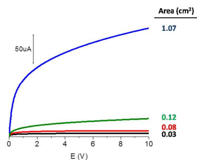
Figure 3: Estimation of electrochemical surface area of the different electrodes ( 0.30 \times 2.50 \text{ mm} ): black (CSPE), red (GRN), green (CSPE modified with PEI), blue (GRN/PEI). Conditions: 3 \mu\text{L} of a dispersion of 0.50 \text{ mg} \cdot \text{mL}^{-1} GRN plus 3 \mu\text{L} of a 100 \text{ mg} \cdot \text{mL}^{-1} polymer preparation.
