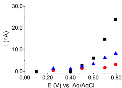
Figure 4: HDVs for 1 mM \text{H}_2\text{O}_2 on GRN/PEI (black) and CSPE (blue). 2 mM D,L-Met on GRN/PEI (red). Other conditions as in Figure 1.
