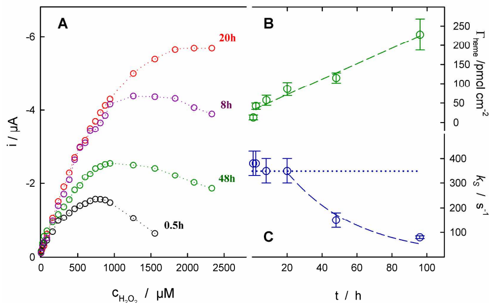
Figure 4. Influence of the indicated incubation time for simultaneous immobilization of r -TOP at graphite electrodes on: (A) voltammetric currents recorded at 0.3 V with v = 0.01 \text{ V s}^{-1} , (B) surface concentration of electroactive heme groups, and (C) their standard electron transfer rate constant. Broken and dotted lines are just eye guides. Other experimental conditions: 0.02M SPB pH 7 and 0°C.
