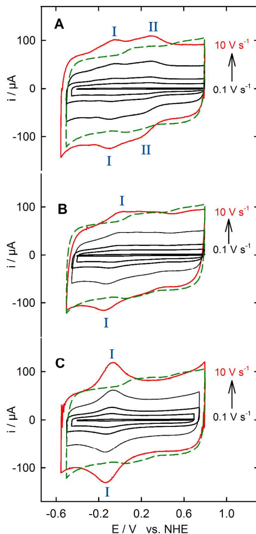
Figure 1. Scan rate dependence of non-turnover cyclic voltammograms recorded in the presence of 0.02M SPB pH 7 at 0°C, corresponding to each of the three protocols of r -TOP immobilization. (A) Physisorption, (B) sequential covalent immobilization and (C) simultaneous covalent immobilization. Scan rates in V s -1 : 0.1, 1, 2, 5 and 10 (red line). The green broken line is a background voltammogram recorded at 10 V s -1 under the same experimental conditions but in the absence of r -TOP. Blue labels I and II help to identify voltammetric peaks associated to r -TOP redox conversion.
