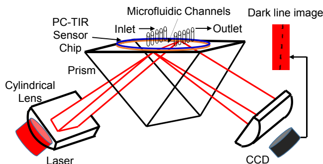
Fig. 1. Schematic diagram of the experimental setup. A microfluidic system is coupled with a PC-TIR sensor. Resonant dark lines of a reflected probe laser beam from the sensor corresponding to the five microchannels can be monitored with a CCD camera.
