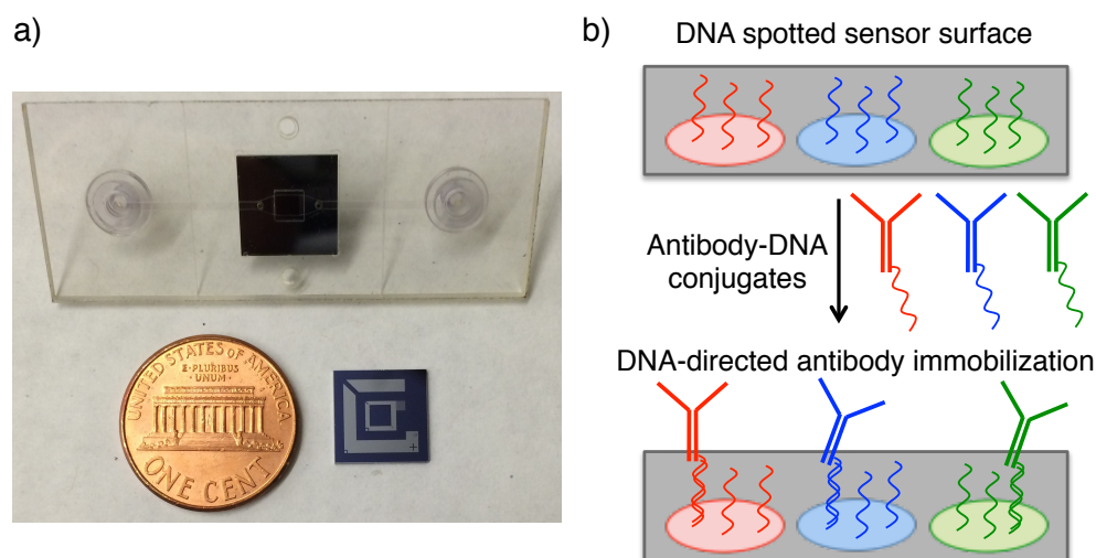
Figure 1. (a) The images of an SP-IRIS chip and an assembled microfluidic cartridge for in-liquid SP-IRIS measurements. (b) A schematic representation of SP-IRIS substrate surface with ssDNA spots and the conversion of this DNA chip into a multiplexed antibody array through hybridization of antibody-DNA conjugates.
