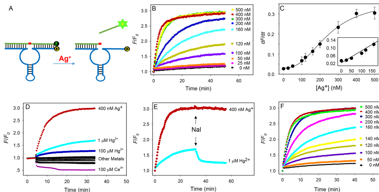
Figure 6. (A) Schematic representation of the Ag + DNAzyme beacon design. (B) Sensor signaling kinetics at various concentrations of Ag + . (C) Quantification of Ag + based on the initial rate of fluorescence enhancement. Inset: the low Ag + concentration region fitted with a linear response. Sensor signaling kinetics with (D) various metal ions: 1 and 100 mM K + , Li + , Rb + , Na + , Cs + ; 1 and 10 mM Ca 2+ , Mg 2+ , 1 and 100 \mu\text{M} Mn 2+ , Fe 2+ , Cu 2+ , Zn 2+ , Ni 2+ , Co 2+ , Cd 2+ , Pb 2+ , Sr 2+ , Ce 3+ , and Fe 3+ . (E) Sensor response to 400 nM Ag + and 1 \mu\text{M} Hg 2+ where the black arrows indicate the time of addition of 10 \mu\text{M} NaI. The fluorescence dropping in the Hg 2+ reaction indicates its signaling was not due to cleavage. All the reactions were performed in 50 mM MOPS, pH 7.5 with 200 mM NaNO 3 . The final sensor concentration was 50 nM. (F) Detecting spiked Ag + in Lake Huron water.
