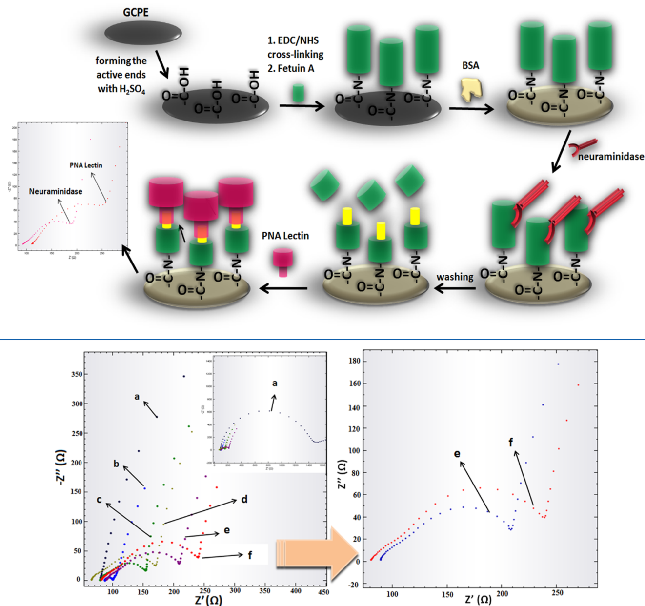
Figure 1. Electrochemical impedance spectra of influenza A model viral biosensor. (a) Plain GCPE, (b) carboxylic groups functionalized GCPE COOH , (c) fetuin A/GCPE COOH , (d) BSA/fetuin A/GCPE COOH , (e) NA/BSA/fetuin A/GCPE COOH , and (f) PNA-Lectin/NA/BSA/fetuin A/GCPE COOH . The EIS procedure was set to measure the electron transfer resistance in frequency range of 0.1 Hz–10 kHz at a potential of 0.25 V and 1 mM K 3 [Fe(CN) 6 ]/K 4 [Fe(CN) 6 ] (in PBS) was used as a redox couple.
