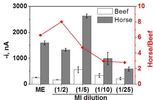
Figure 7. Amperometric responses measured with the developed electrochemical DNA sensor in the analysis of mitochondrial DNA extracted (ME) from 3.0 g of beef and horse meat and directly in the raw mitochondrial lysates (MI) obtained from the same amount of meat diluted different times with blocker casein solution. Error bars were estimated as triple of the standard deviation ( n=3 ).
