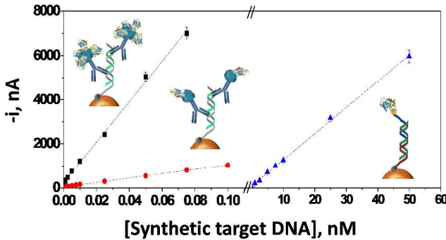
Figure 3. Calibration plots obtained for the synthetic target DNA with the developed sensor (in black), using ProtA-HRP instead of ProtA-HRP40 for enzymatic labeling (in red) and with a sandwich conventional strategy (in blue). Error bars were estimated as triple of the standard deviation (n=3).
