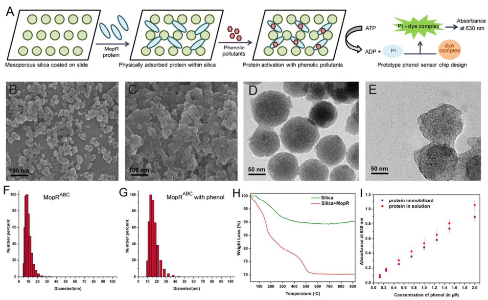
Figure 3. Design and characterization of protein sensor chip. (A) Schematic representation of the MopRABC protein based biosensor strip design. The external particle morphology of the spherical MCM-41 before and after protein adsorption were ascertained by SEM images (B) MCM-41 and (C) MCM-41 with adsorbed protein. TEM images of (D) MCM-41 and (E) MCM-41 with adsorbed protein (F-G) DLS size distribution analysis of MopRABC in native (F) and phenol bound (G) form. (H) TGA curves of MCM-41 silica before and after MopRABC protein adsorption. (I) Sensitivity plot for the immobilized MopRABC protein. Both protein in solution and immobilized format retained similar sensitivity, especially at lower concentrations.
