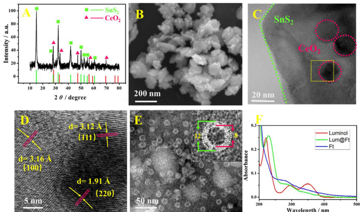
Figure 1. XRD pattern (A), SEM image (B), TEM image (C), and HRTEM image (D) of \text{CeO}_2/\text{SnS}_2 heterostructures. TEM image (E), and HRTEM image (inset) of a single Ft. UV-vis spectra (F) of Ft, luminol, and Lum@Ft.
