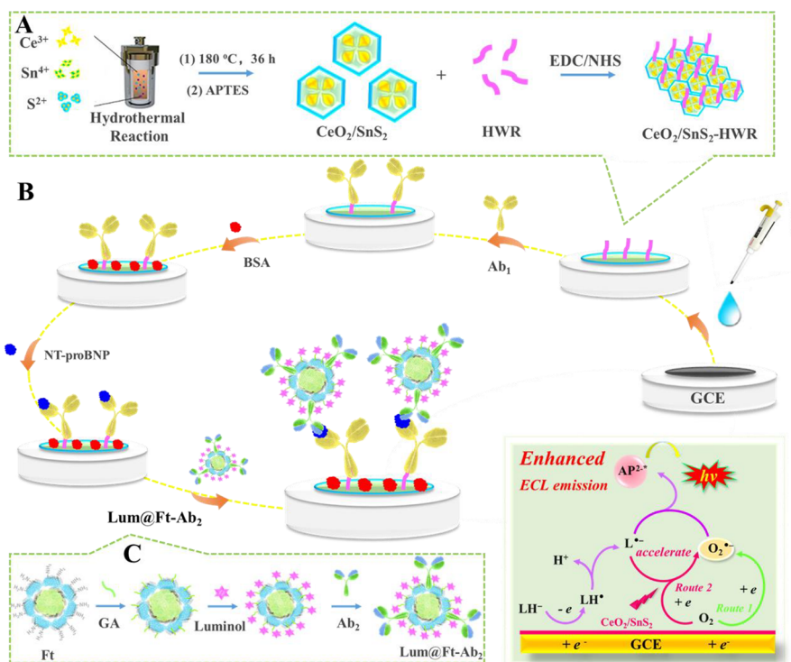
Scheme 1. (A) Graphical Expression of \text{CeO}_2/\text{SnS}_2 –HWR Preparation, (B) Diagram of the Fabrication Process and Possible Mechanism of the Biosensor, and (C) Preparation Procedure of \text{Lum@Ft-Ab}_2 Bioconjugate
