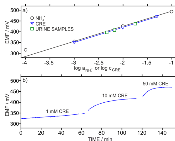
Figure 4. (a) Calibration graphs observed for ammonium and creatinine in the microfluidic cell illustrated in Figure 1. The potentials registered for the three urine samples are also shown. (b) Dynamic response of the ammonium-selective electrode at increasing concentration of creatinine, using the microfluidic cell illustrated in Figure 1.
