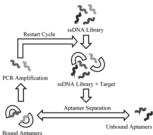
Figure 3. SELEX cycle starts with incubation of target bioanalyte with oligonucleotide. Unbound aptamers are removed retaining only bound aptamer sequences for PCR amplification to regenerate the oligonucleotide library and restart cycle.
