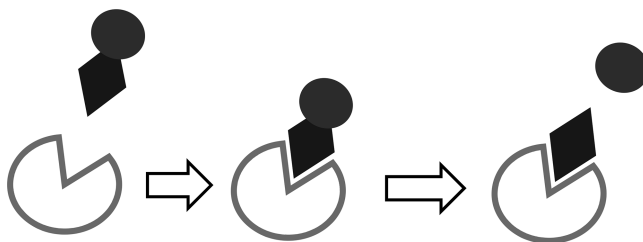
Figure 2. Target bioanalyte binds active site (left) to form bioanalyte-enzyme complex (middle) where a catalytic reaction converts target bioanalyte to measurable reaction product (dark circle, right).
