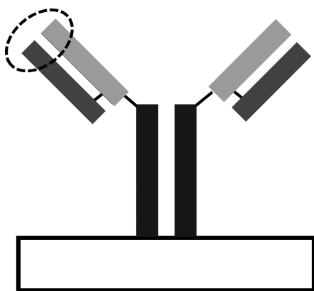
Figure 1. 3D confirmation of antibodies is “Y” shaped with binding domains, circled above, typically located on the distal end.
