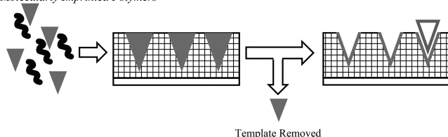
Figure 4. Synthetic polymerization encapsulating the target bioanalyte forms an analyte binding site.
