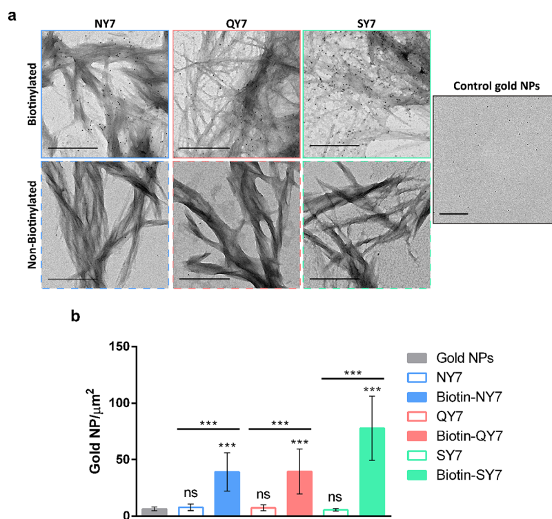
Figure 2. Characterization of biotinylated NY7, biotinylated QY7, and biotinylated SY7 amyloid scaffolds incubated with streptavidin-gold NP conjugates. (a) TEM micrographs of biotinylated NY7 (blue), biotinylated QY7 (red), and biotinylated SY7 (green) peptides were prepared at 250 \mu\text{M} to a 1:5 (biotinylated peptide:nonbiotinylated peptide) ratio, corresponding to the top-line images with continuous lines. Dashed lined images at the bottom correspond to nonbiotinylated scaffold controls. Streptavidin-gold NP conjugate control corresponds to the right image (black continuous line). Scale bars correspond to 500 nm. (b) Quantification of gold NPs. TEM micrographs acquired in panel (A) were used to quantify gold NPs, and the content was expressed as numbers of gold NPs/ \mu\text{m}^2 . Data correspond to the average quantification from at least five micrographs from two independent experiments, and bars correspond to the SD of the mean. For all peptides, the one-way ANOVA statistical test was performed relative to the gold NP control (** P -value < 0.001, ** P -value < 0.01, and * P -value < 0.05) followed by a Bonferroni's multiple comparison test (** P -value < 0.001, ** P -value < 0.01, and * P -value < 0.05) to compare biotinylated and nonbiotinylated samples.
