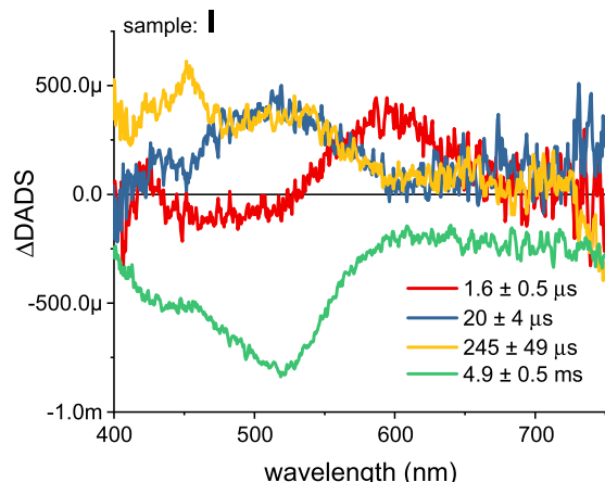
Figure 5. \Delta DADS for sample I obtained by subtracting RC contributions from the DADS in Figure 4. Subtraction was performed primarily to reveal the formation of the oxidized form of the polymer.
