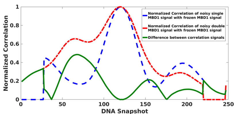
Figure 6. Counting the number of proteins: To count the number of proteins, we consider the normalized correlations between the frozen single MBD–DNA complex and the noisy signals from the translocation of the DNA with a single-MBD (blue) and multiple-MBD (red). A difference (green) between the two aligned correlation peaks results in the presence of a peak, the value of which can be used to determine the presence or absence of the second protein depending on a preset threshold value.
