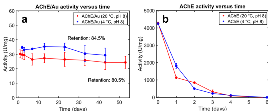
Figure 5. (a) Activity retention of AChE immobilized on bare gold and (b) in solution and stored at either 20 °C (red) or 4 °C (blue). ATCh concentrations were 0.5 mM in both cases. The AChE solution concentration was 10 nM. Error bars indicate a standard deviation of three measurements. The same set of samples was measured at each subsequent time point.
