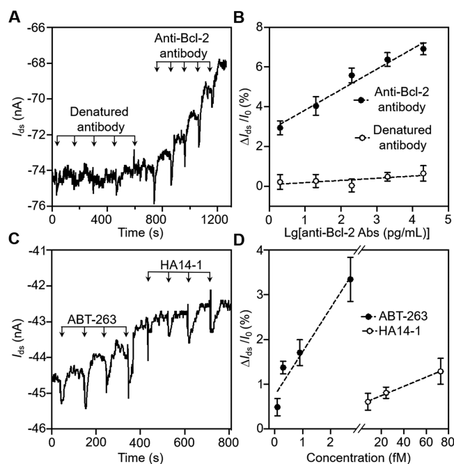
Figure 5. Detection of OMM-reactive compounds by OMM-FETs. (A,B) Anti-Bcl-2 antibodies and (C,D) ABT-263 and HA14-1, two small molecule Bcl-2 inhibitors, were used as model molecules for the test. OMM-FETs were used to measure the channel conductance as more antibodies and inhibitors were added to the OMM-FET surface. Typical I_{ds} -time curves of the compounds (A,C) were measured and values of I_{ds} that changed relative to the basal level ( \Delta I_{ds}/I_0 ) were plotted against compound concentrations (B,D). In B and D, the error bars were obtained by randomly picking 30 time points from the plateau of the I_{ds} -time curves after adding each molecule; mean \pm standard deviation.
