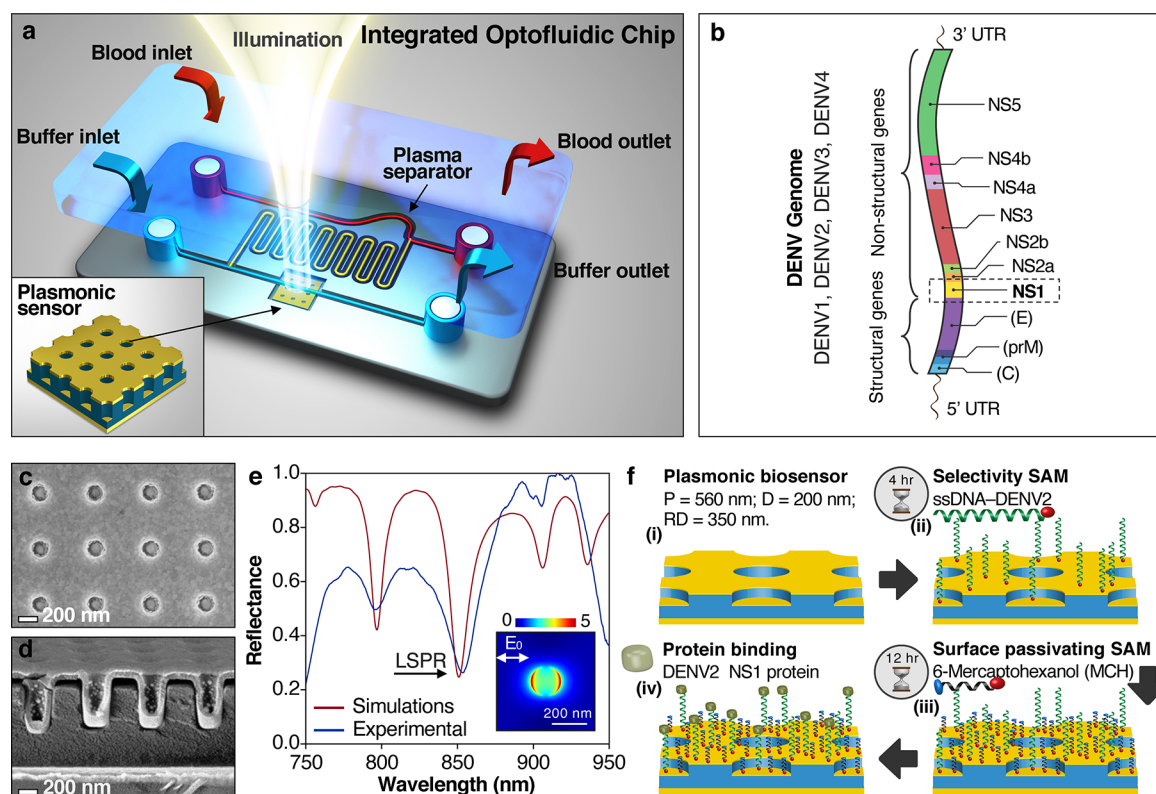
Figure 1. (a) Integrated Dengue virus biosensor comprising an in-line microfluidic blood plasma separator and a cavity-coupled nanoimprinted plasmonic array. Inset corresponds to the nanoimprinted plasmonic biosensor composed of a gold mirror (80 nm), a dielectric film spacer ( \sim 700 nm) embossed with a square array of holes, a conformal thin film of aluminum oxide layer (20 nm) as fluid barrier, and a thin gold film (30 nm). (b) Dengue virus genome shared among the four DENV serotypes and comprised of three structural (C, prM, and E) and seven nonstructural (NS) proteins, including NS1. (c,d) Scanning electron microscope images, top view (c) and cross section (d), of one representative nanoimprinted sensor. (e) Reflectance spectra obtained using FDTD simulations (red curve) and experimentally (blue curve). Inset represents the electric field enhancement obtained 5 nm above the circular hole at the LSPR. (f) Representation of the biosensing workflow. (i) The sensors are batch prepared and properly cleaned prior to functionalization. (ii) Thiol-terminated ssDNA aptamer specific to nonstructural DENV2-NS1 protein binds covalently to the gold surface. This step requires incubation for 4 h. (iii) Thiol-terminated 6-mercaptopentanol (MCH) self-assembly monolayer binds covalently to the empty surface area to block nonspecific binding and decrease protein fouling present in biological fluids. This process requires incubation for 12 h. (iv) DENV2-NS1 protein detection via aptamer binding, which produces a readable LSPR shift.
