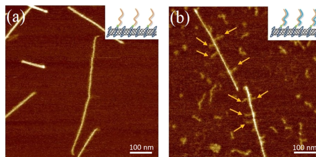
Figure 2. AFM images, and cartoon insets, of aptamer-functionalized SWCNTs (a) without and (b) with hybridized ss-DNA sequences. The yellow arrows show the hybridized aptamers along the nanotubes. Z-scales = 2.5 nm.
