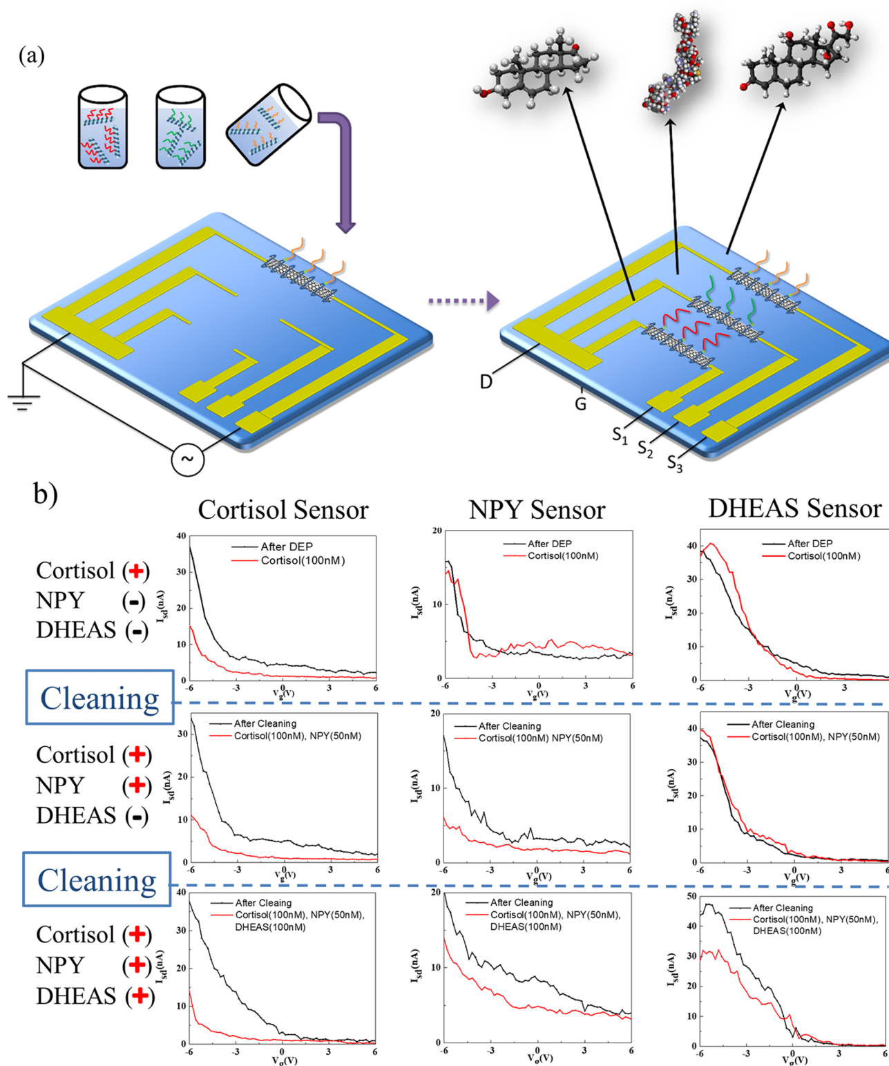
Figure 4. (a) Schematic of the DEP strategy employed for the fabrication of multisensing devices: a drop of the chosen SWCNT-aptamer solution is cast on the chip mainly over one electrode pair, a voltage is then applied only across this electrode pair in order to direct the assembly of SWCNT-aptamer hybrids only across this pair of electrodes, and not the others (see also the SI); (b) multiplexed sensing: electrical responses of the different biosensors on the same chip ( V_{sd} = 100 mV): the + sign indicates the addition/presence of the analyte of interest; the "cleaning step" indicates the addition of 8 M of urea in order to regenerate the sensor after each detection; "after cleaning" indicates the measurements performed after this step.
