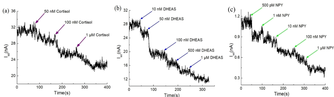
Figure 5. Real time detection of (a) cortisol (from 50 nM to 1 \mu M), (b) DHEAS (from 10 nM to 1 \mu M), and (c) NPY (from 500 pM to 1 \mu M) at various concentrations, in serum ( V_{sd} = 100 mV, V_g = -2 V).
