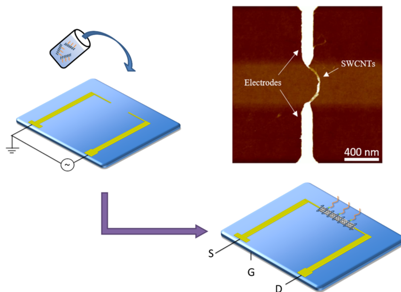
Figure 3. DEP of SWCNT-aptamer hybrids with the corresponding AFM picture. S, D, and G respectively indicate the source, drain, and gate (electrodes); Z-scales = 10 nm.
