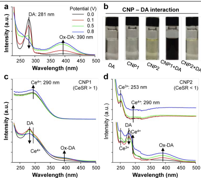
Figure 2. CNP-dopamine interaction analysis in-situ. (a) Dopamine UV-visible spectro-electrochemical analysis as a function of external potential: 0, 0.1, 0.5 and 0.8 V. (b) Optical images of dopamine and its interaction with CNP1 (CeSR > 1) and CNP2 (CeSR < 1). UV-visible spectro-electrochemical analysis of pristine (top) and mixed with dopamine (bottom) for CNP1 (c) and CNP2 (d) as a function of oxidizing potential: 0, 0.1, 0.5 and 0.8 V.
