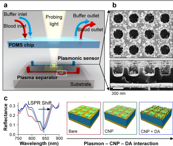
Figure 1. Integrated enzyme-free dopamine sensing. (a) Schematic representation of the integrated device comprised of a plasmonic sensor coupled to a microfluidic chip containing the plasma separator module. (b) Top view and cross section SEM of one CNP-functionalized plasmonic substrate. (c) Experimental spectra of one fabricated device (red), its spectral response after CNP coating (green) and after DA incubation at one representative concentration (blue). Right panels represent graphically these three phenomenological events.
