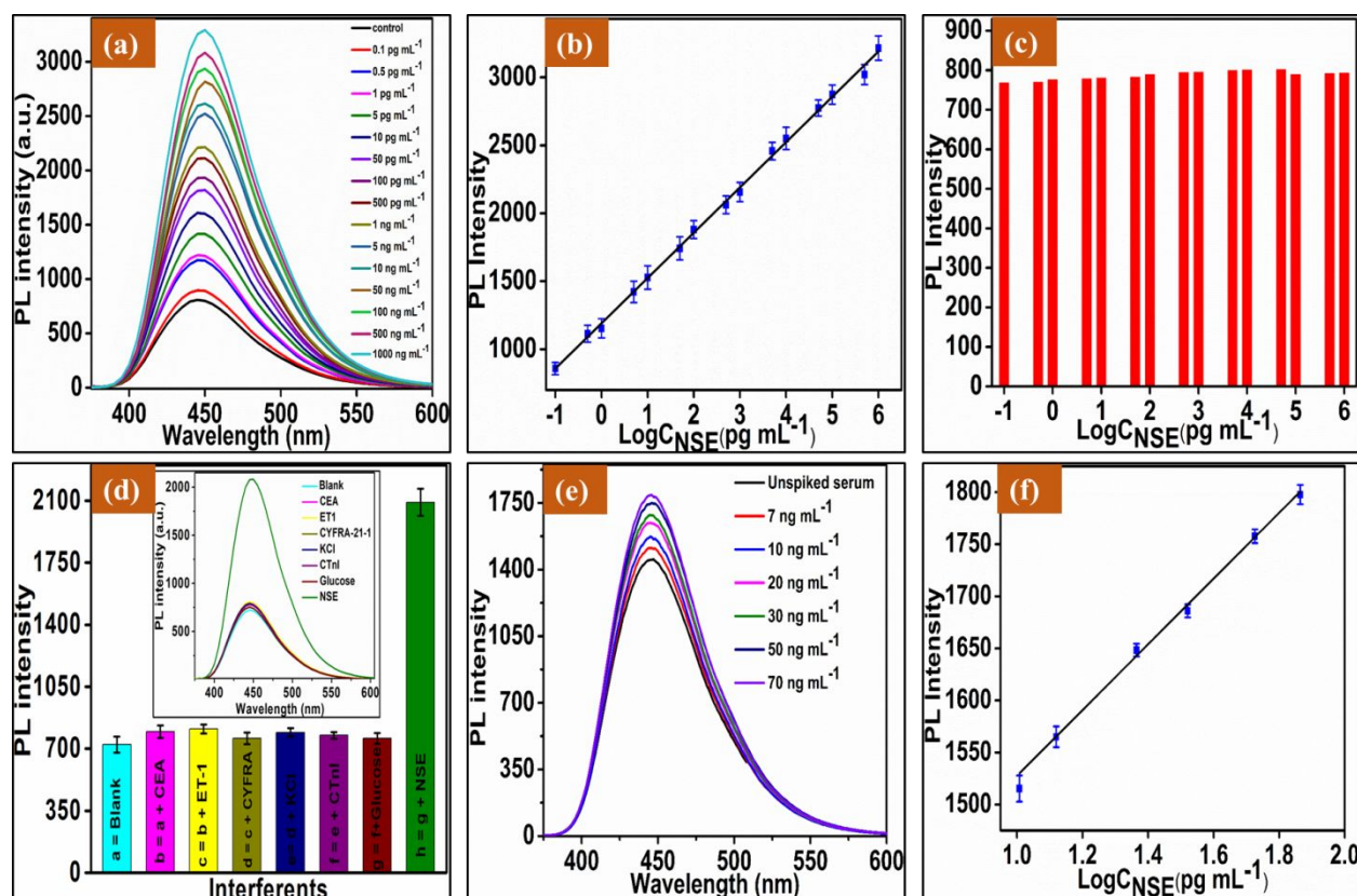
Figure 5: (a) Fluorescence response studies of anti-NSE/amine-N-GQDs@AuNPs nanoprobe as a function of NSE antigen concentration (0.1 pg mL -1 to 1000 ng mL -1 from bottom to top); (b) The calibration curve indicating the linear relationship between log concentration of NSE and PL intensity of the nanoprobe; (c) Control experiment of amine-N-GQDs@AuNPs as a function of log concentration of NSE antigen and PL
