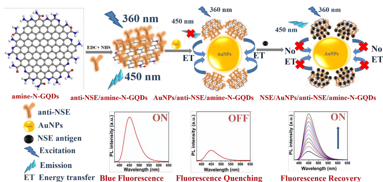
Figure 1. Pictorial representation indicating the mechanism of the fluorescent biosensor
