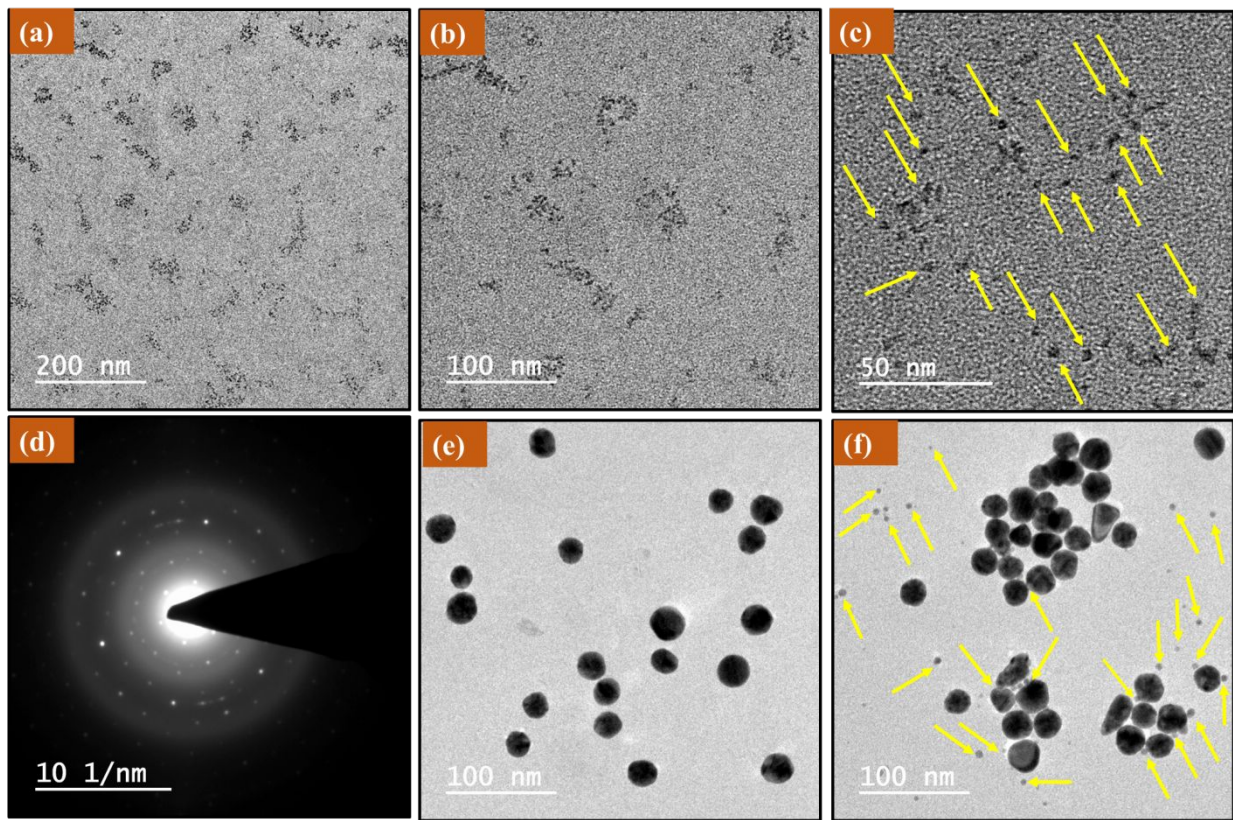
Figure 2: (a-c) TEM image of synthesized amine-N-GQDs at different scales; (d) SAED pattern of amine-N-GQDs; (e) TEM image of AuNPs (f) TEM image of the amine-N-GQDs@AuNPs composite.
