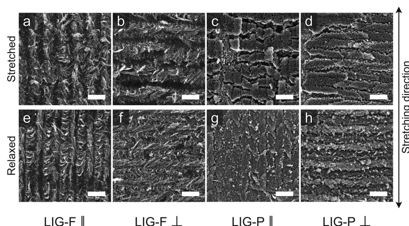
Figure 4. Effect of stress on LIG/MPU. SEM images of samples under stretching: (a) LIG-F ||, (b) LIG-F ⊥, (c) LIG-P ||, and (d) LIG-P ⊥. (e–h) Corresponding images of relaxed samples after 200 cycles of 30% strain. Scale bar: 100 \mu m.
