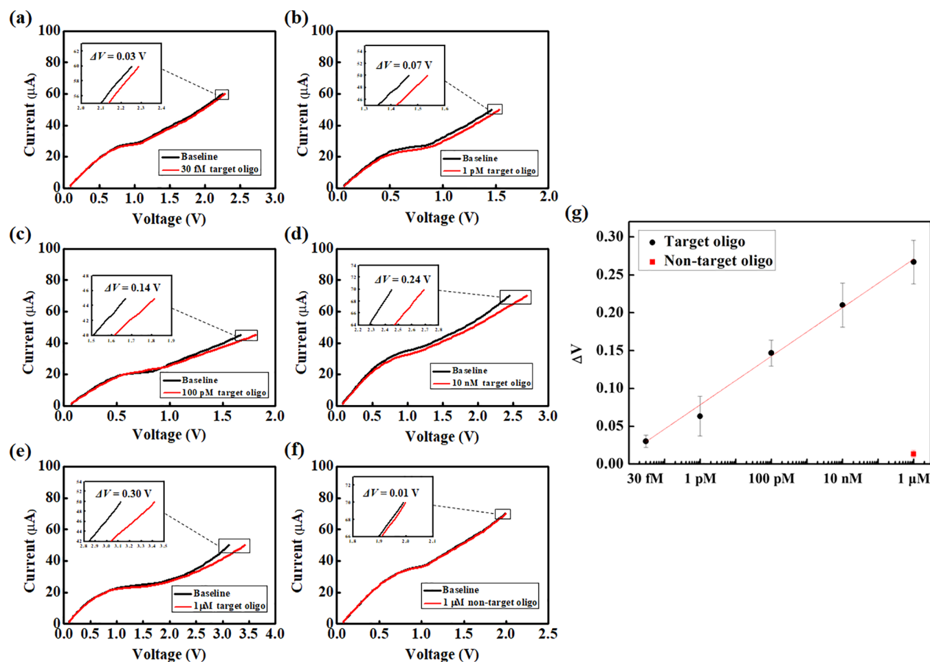
Figure 13. Voltage shift blow-up of target gene oligo in a range from 30 fM to 1 \mu\text{M} with the HDA-4 membrane sensor in the CVC measurements and the blow-up with 1 \mu\text{M} nontarget gene oligo.
