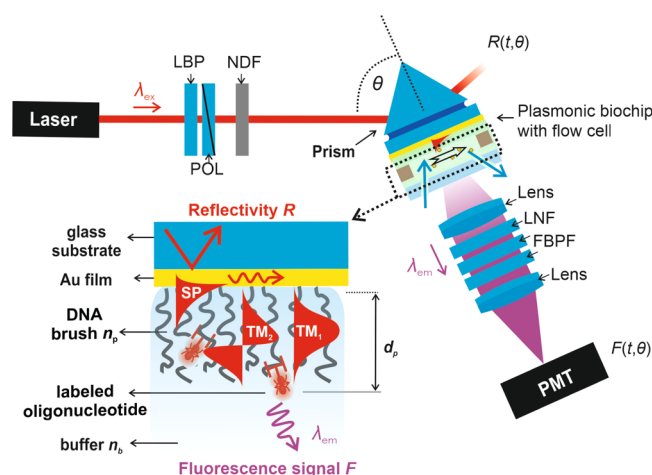
Figure 1. Optical configuration used for the combined SPR, OVS, and SPFS measurements.
