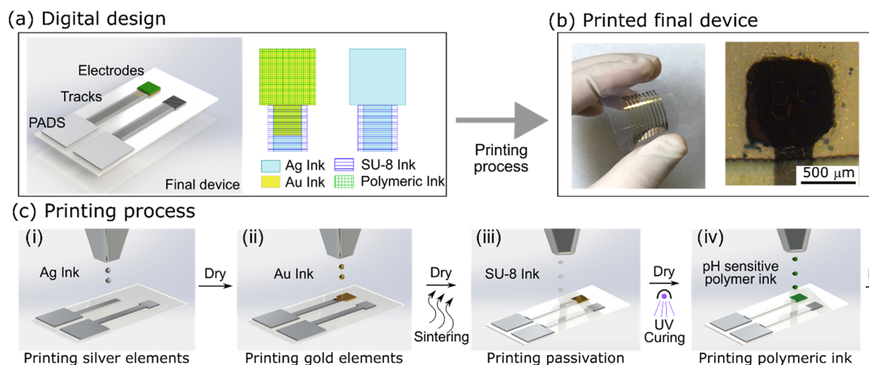
Figure 1. (a) Digital design of the pH sensor. (b) Final printed platform with 9 IE and 1 pRE and microscopic image of the printed polymeric electrodes. (c) Inkjet printing steps: (i) printing of Ag RE, tracks, and pads, followed by a dry step; (ii) printing of the Au IE, followed by a dry and thermal sintering of both metallic Au and Ag layers; (iii) printing of the dielectric SU-8, drying, and UV cross-linking; and (iv) printing of CP inks, followed by a drying step.
