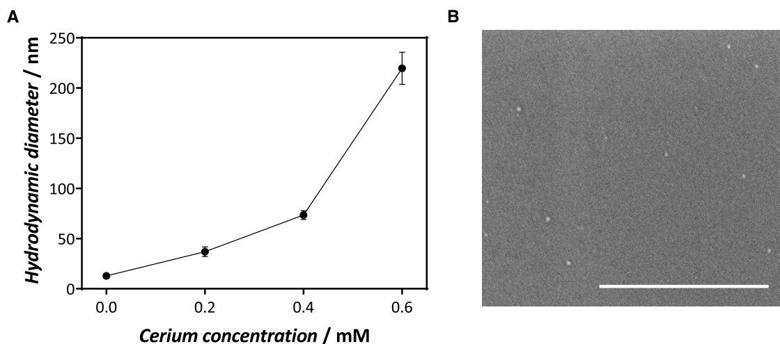
Figure 2. Characterization of Ce@pGOx_3 hybrids. (A) Hydrodynamic diameters measured by DLS for the hybrids assayed. (B) SEM pictogram of Ce@pGOx_3 hybrid synthesized from 0.2\text{ mM} of \text{Ce}^{3+} (scale bar: 400\text{ nm} ).
