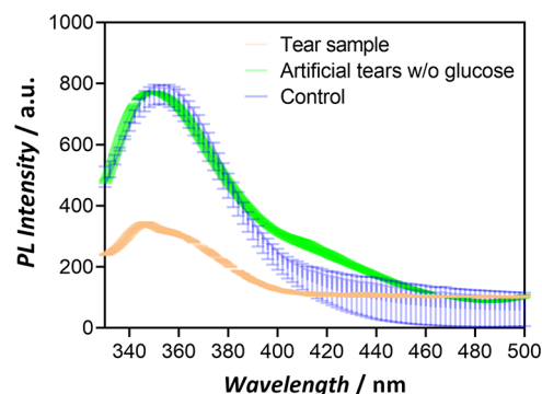
Figure 6. Photoluminescence spectra of Ce@pGOx in the presence of a solution with and without glucose at 40 \mu M .
