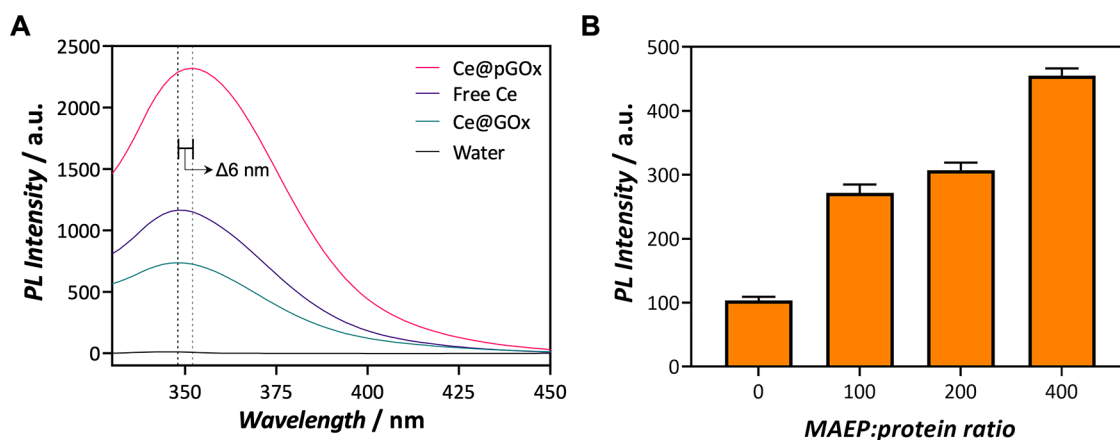
Figure 3. Photoluminescence analysis of the hybrids ( \lambda_{\text{exc}} 310 nm). (A) Fluorescence emission spectra of the hybrid nanogels synthesized with and without phosphate groups (Ce@pGOx and Ce@GOx, respectively) and a free cerium solution at 0.2 mM. (B) Fluorescence intensity values recorded for Ce@GOx_0-3 samples assembled with 0.2 mM of Ce(III).
