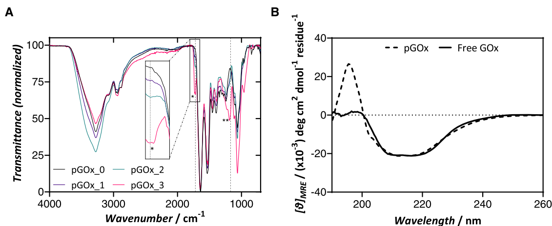
Figure 1. Characterization of pGOx nanogels. (A) ATR-FTIR spectra of nanogel samples. Characteristic bands, 1723\text{ cm}^{-1} (*) and inset zoom in) and 1170\text{ cm}^{-1} (**), reveal the presence of phosphates within the pGOx_1 to 3 nanogels. (B) Circular dichroism spectra in the far-UV spectrum of unmodified and encapsulated GOx enzyme.
