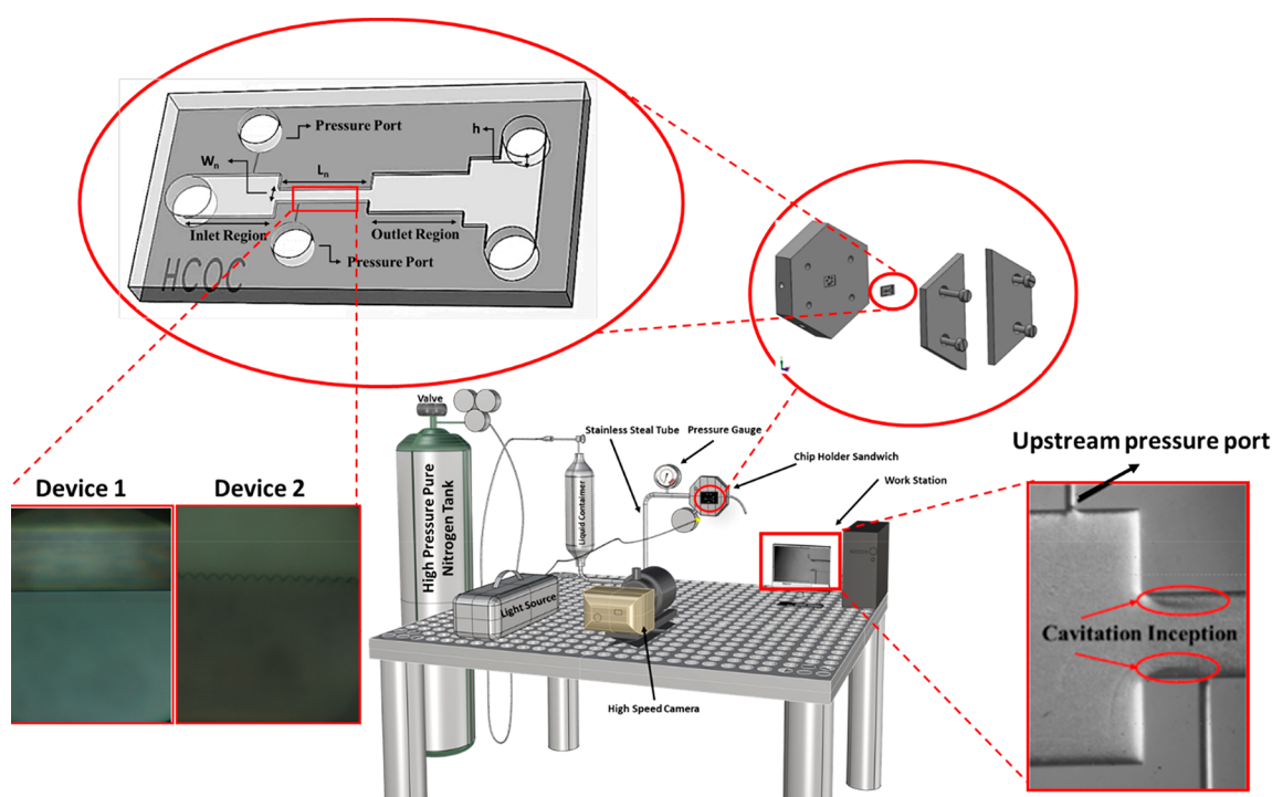
Figure 2. Experimental setup and microfluidic chip details. The cavitation inception is detected using the high-speed camera, and the pertinent pressure to the instance of cavitation inception is recorded as the cavitation inception pressure.
