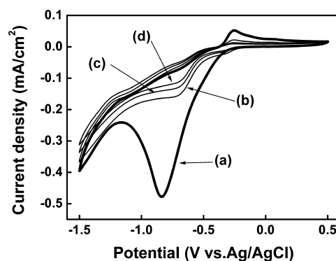
Figure 4. Cyclic voltammograms of reduction of nitrophenyl films on ZnO in solution ( C_2H_5OH-H_2O (V/V = 1:9)) containing 0.1 M KCl; scanning rate, 100 mV s -1 . (a) First scan; (b)–(d) second to fourth scans.
