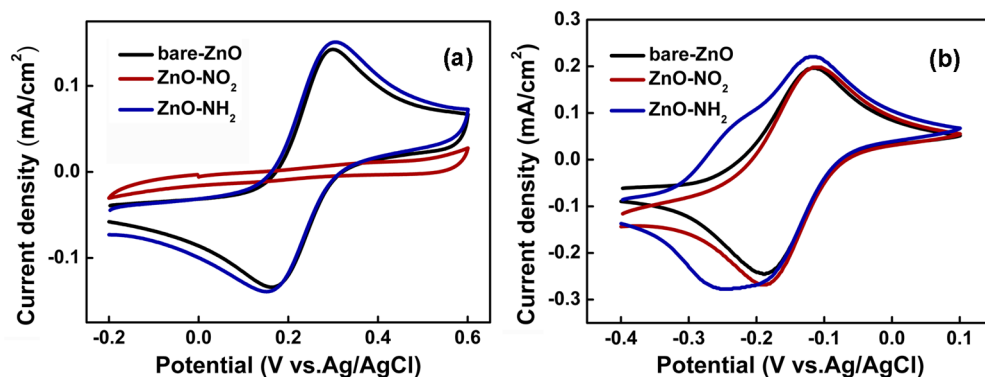
Figure 7. Cyclic voltammograms in 1 mM \text{Fe}(\text{CN})_6^{3-/4-} (a) and 1 mM \text{Ru}(\text{NH}_3)_6^{2+/3+} (b) solution of bare ZnO film, 4-nitrophenyl layers on ZnO (ZnO- \text{NO}_2 ), and after reduction of 4-nitrophenyl groups on ZnO (ZnO- \text{NH}_2 ).
