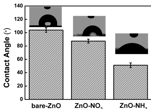
Figure 6. Contact angles of a bare ZnO film, 4-nitrophenyl layers coated ZnO (ZnO- \text{NO}_2 ), and after the reduction of 4-nitrophenyl groups on ZnO (ZnO- \text{NH}_2 ).
