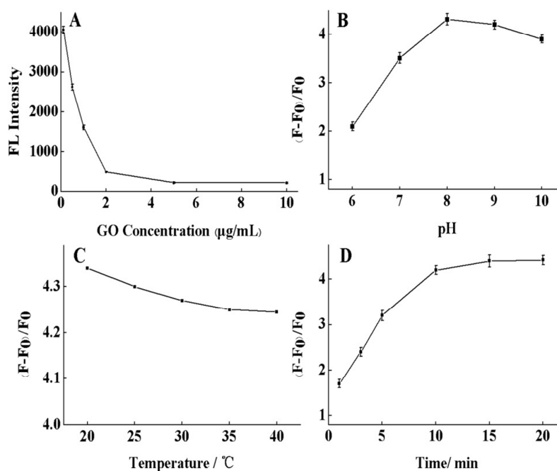
Figure 2. Influence of the relevant experimental factors on the fluorescence intensity of sensing system. (A) GO concentration, (B) pH values, (C) temperature, (D) reaction time: FAM-ssDNA for A, B, C and D, 10 nM. BPA for B, C and D, 10 ng/mL. GO for B, C and D, 2 μg/mL.
