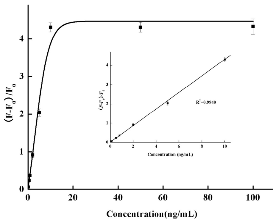
Figure 4. The peak fluorescence change ((F-F_0)/F_0) as a function of BPA concentration. Inset: the peak fluorescence of change is linear with BPA concentration over the range from 0.1 ng/mL to 10 ng/mL. \lambda = 494 nm.
