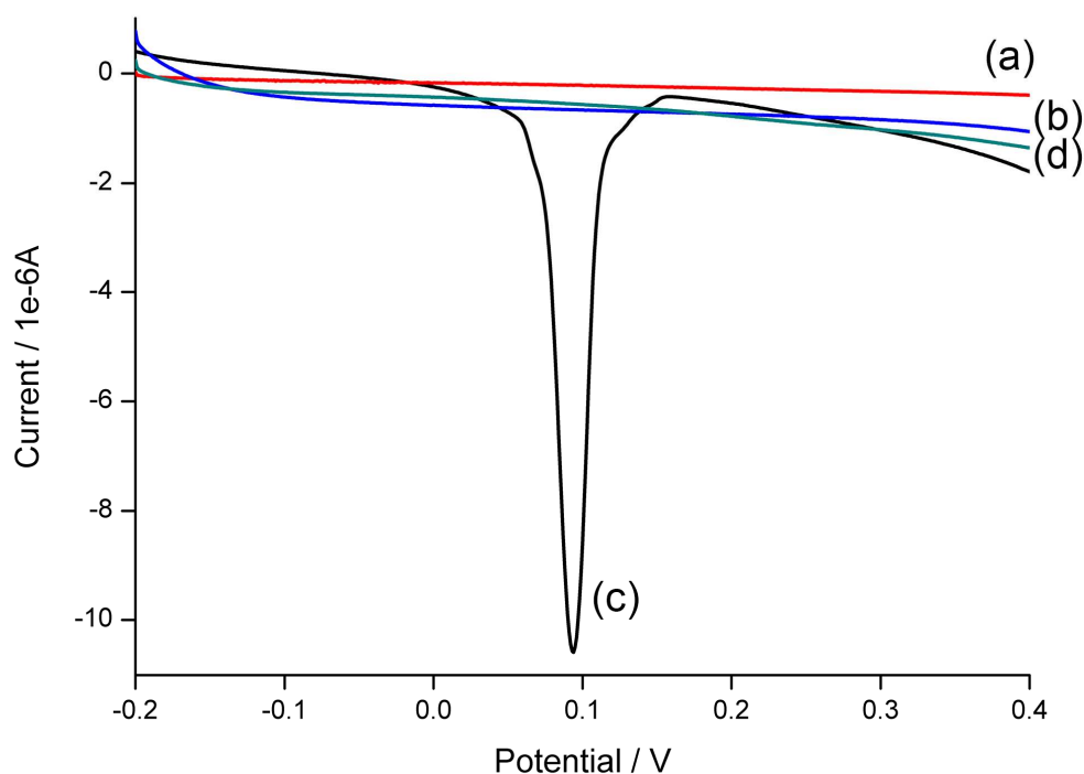
Figure 3. Linear sweep voltammograms of (a) bare gold electrode, tetrahedral DNA nanostructure modified electrode after strand displacement reaction in the (b) absence and (c) presence of 100 fM microRNA, (d) is the case in the presence of 100 fM microRNA using signal probe without AgNPs labels.
