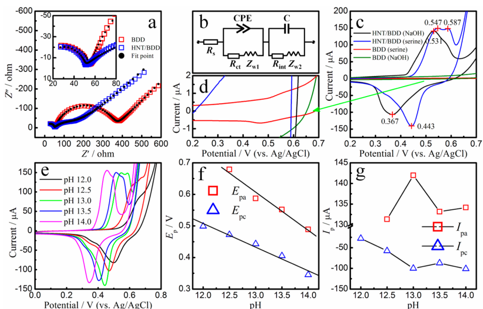
Figure 5. (a) Nyquist plots of the EIS for the bare BDD (red) and Ni–NiO HNT/BDD (blue) electrodes in 0.1 M KCl containing 5 mM [\text{Fe}(\text{CN})_6]^{3-/4-} with a frequency range of 0.01\text{--}1 \times 10^6 Hz and signal amplitude at 0.005 Hz. The inset shows the expanded high-frequency region of the plots (symbols, experimental data; black points, fitting results). (b) The equivalent circuit for data fitting. R_s , the electrolyte resistance; R_{ct} , the charge-transfer resistance at the electrode/electrolyte interface; Z_{W1} , the Warburg impedance accounting for the ion diffusion; CPE, resistance at the Ni–NiO HNT and the double-layer capacitance at the BDD interfaces; R_{inv} , the Faradaic reaction impedance at the electrode/electrolyte interface; Z_{W2} , the Warburg impedance accounting for diffuse ion storage at low frequency in the electrode/electrolyte interface; C , capacitance at the Ni–NiO HNT/BDD interface. (c) CV responses of the BDD (red and green) and the Ni–NiO HNT/BDD (blue and black) electrodes at a scan rate of 100 \text{ mV s}^{-1} in a 0.1 M NaOH (pH 13.0) solution with and without 0.1 mM \text{L-serine} . (d) Enlarged CV curve for the bare BDD (red) in a 0.1 M NaOH (pH 13.0) solution with 0.1 mM \text{L-serine} . (e) CVs of the Ni–NiO HNT/BDD electrode in \text{N}_2 -saturated NaOH solutions of different pH: 12.0 (black), 12.5 (red), 13.0 (green), 13.5 (blue), and 14.0 (pink), with a scan rate of 100 \text{ mV s}^{-1} . (f) Plot of the anodic ( E_{pa} ) and cathodic peak ( E_{pc} ) potentials vs pH values. (g) Plot of the anodic and cathodic peak currents vs pH values.
