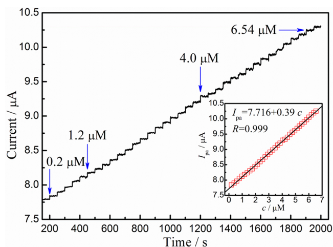
Figure 7. Amperometric response of the Ni–NiO HNT/BDD electrode during successive additions of L -serine into air-saturated, stirred NaOH (0.1 M, pH 13.0) at an applied potential of 0.59 V. The inset presents the calibration curve for the L -serine concentration obtained by the biosensor (symbols, experimental data; line, fitting results).
