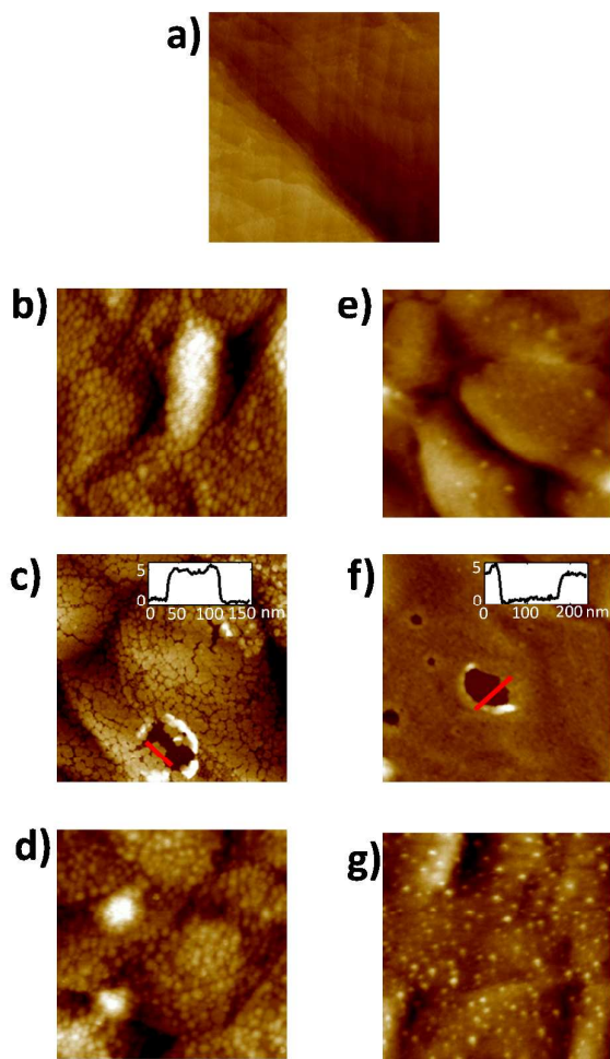
Figure 2. Atomic force microscopy topography images of clean, HFBI-Z E and HFBI-Protein A receptor module layers on CVD graphene on platinum. a) Clean graphene surface on platinum before any functionalization. b) Surface after HFBI-Z E functionalization in 100 mM pH 7 NaP buffer, c) after drying in N 2 and d) after re-wetting in the buffer. e) Surface after HFBI-Protein A functionalization in 100 mM pH 7 NaP buffer, f) after drying and g) after re-wetting in the buffer. For both of the receptor modules protein film shrinkage and possible mechanical forces during the drying tend to create cracks in the film but damage is healed in both cases after 5 min re-wetting in the buffer. The height profiles of the dried samples in the insets of figures c) and f) correspond to the red lines in the same figures. The thickness of both the dried HFBI-Z E and HFBI-Protein A layers is 4 to 5 nm, corresponding to a typical thickness of a monomolecular fusion protein layer after drying. The image size is 1 x 1 \mu\text{m}^2 and height scale 15 nm in all the images.
