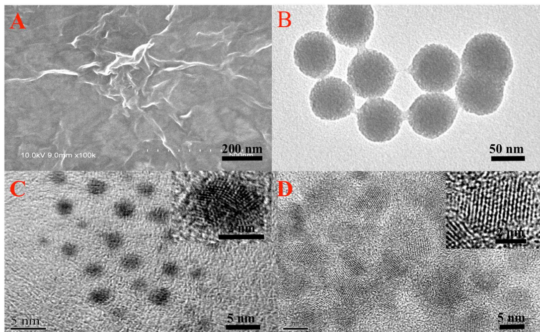
Figure 1. (A) SEM image of reduced graphene oxide, (B) TEM image of SmS NPs, (C) HRTEM image of Ag NCs, and (D) HRTEM image of CdSeTe@CdS QDs.
