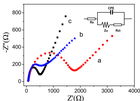
Figure 2. Electrochemical impedance spectra of the bare GCE (a), MMPF-6(Fe)/GCE (b), and AuNPs/MMPF-6(Fe)/GCE (c) in 0.1 mol L -1 KCl solution containing 5 mmol L -1 [\text{Fe}(\text{CN})_6]^{3-/4-} .
